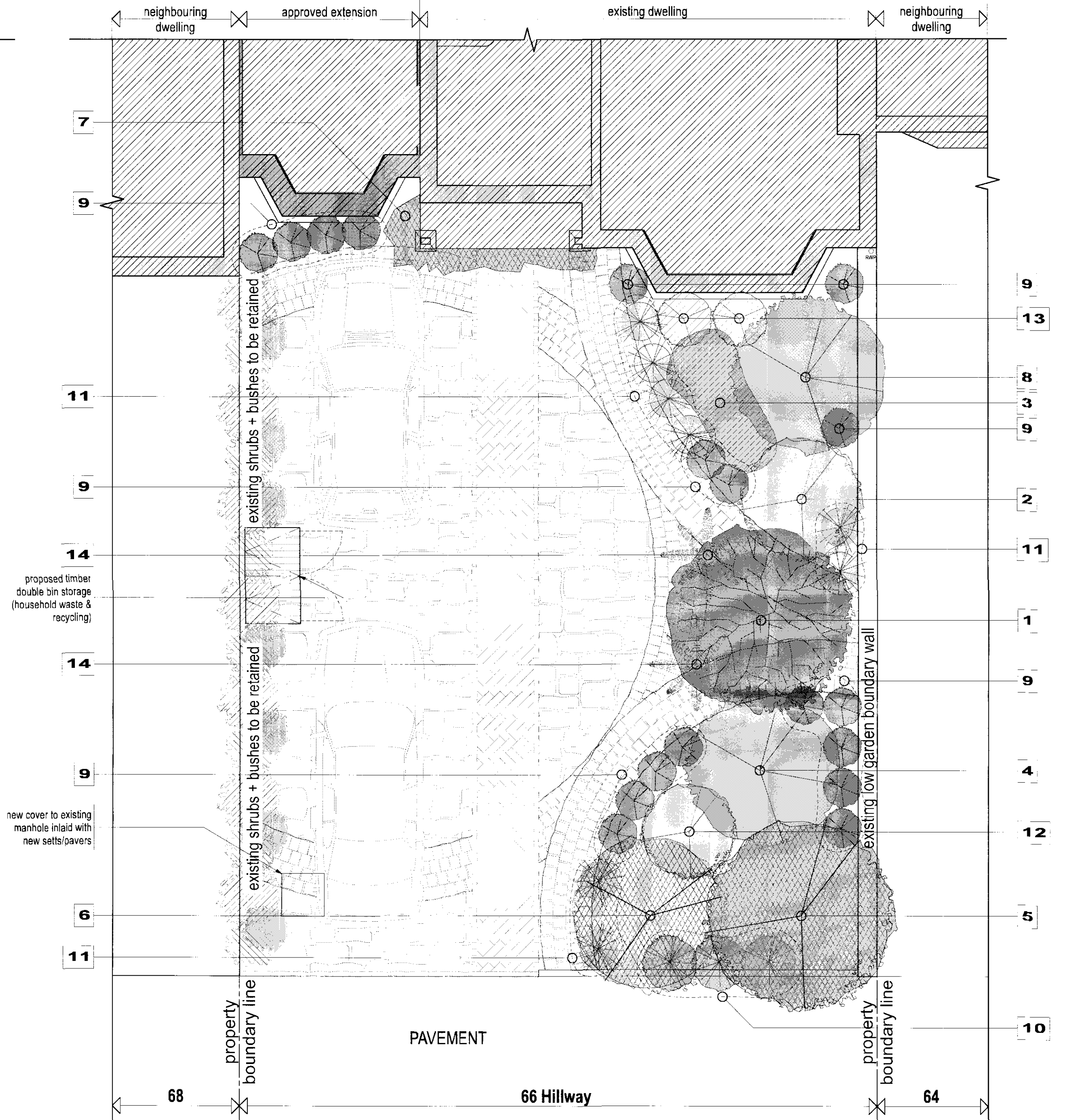
front garden landscape plan: proposed
