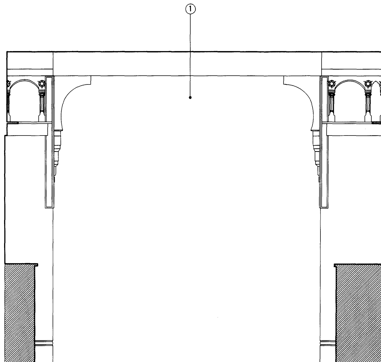
NORTH WALL
