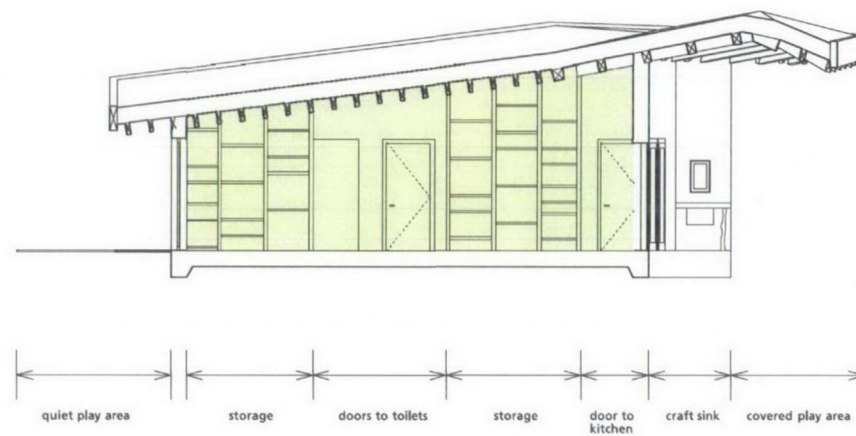
03 long section looking east approved 1:100
