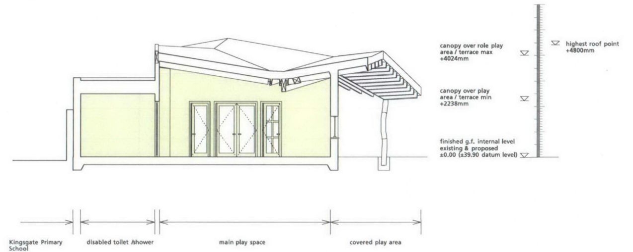
04 short section facing south approved 1:100
