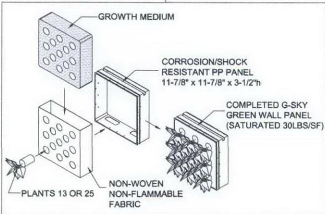
G-SKY GREEN WALL PANEL ASSEMBLY
