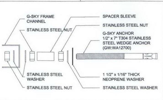
G-SKY ANCHOR DETAIL
