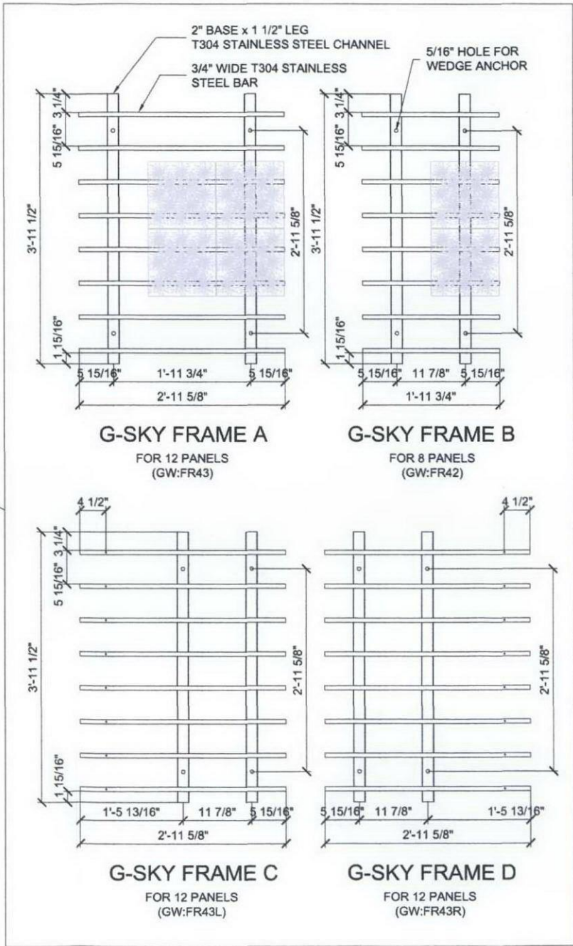
G-SKY FRAME DETAILS
