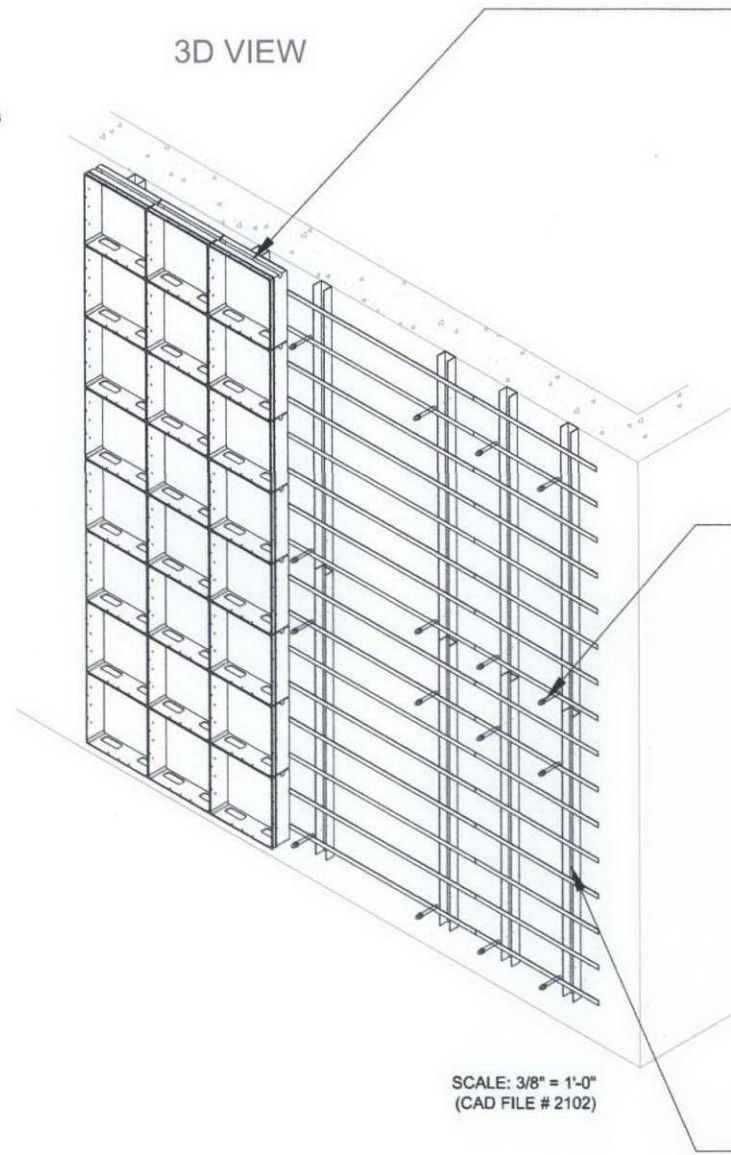
G-SKY ANCHOR DETAIL
