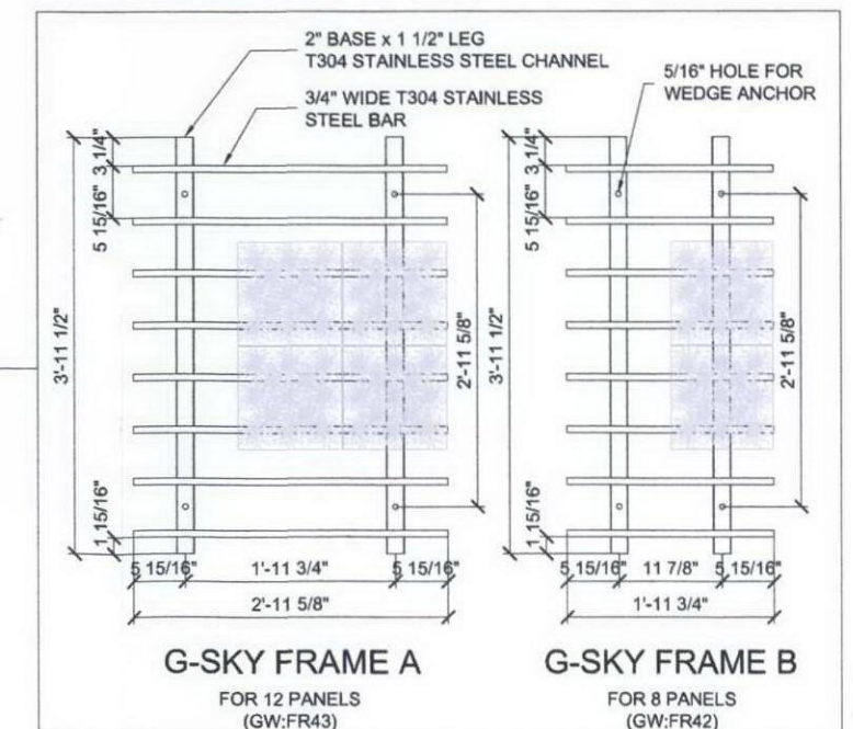
G-SKY FRAME DETAILS
