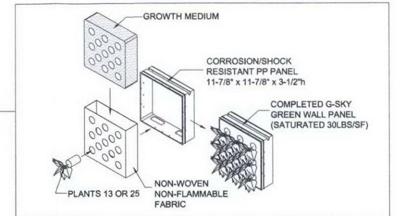
G-SKY GREEN WALL PANEL ASSEMBLY
