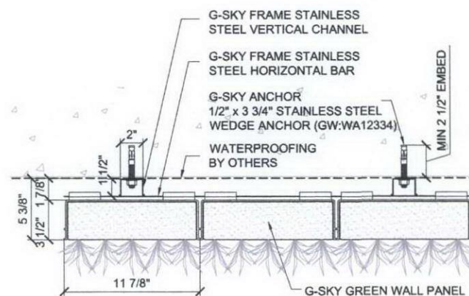
PLAN SECTION
