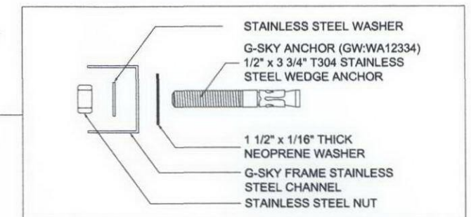
G-SKY ANCHOR DETAIL
