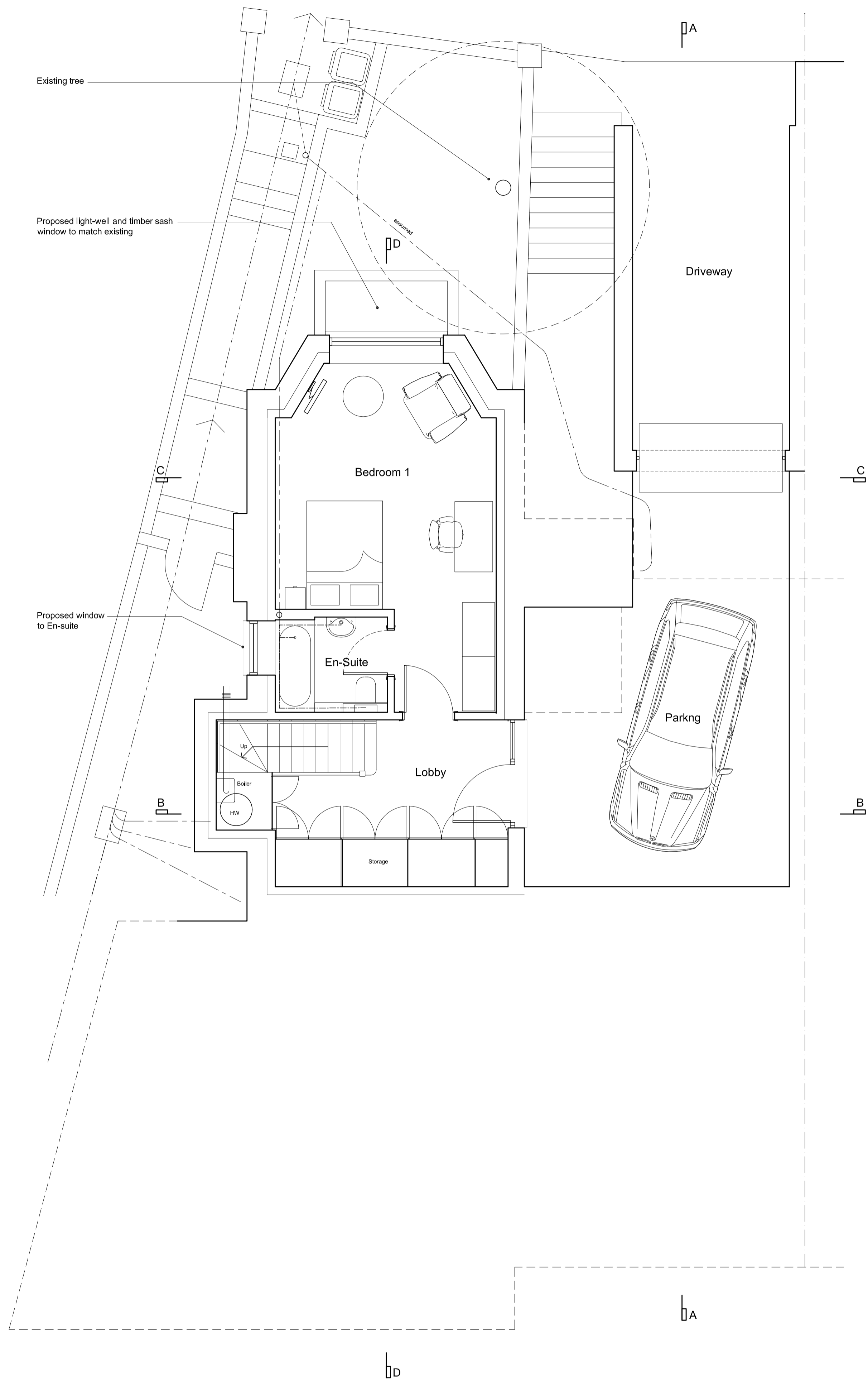
Lower Ground Floor 1:50
