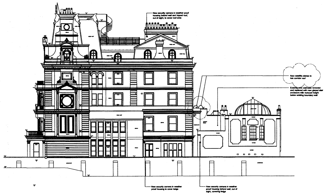
1 SIDE ELEVATION
