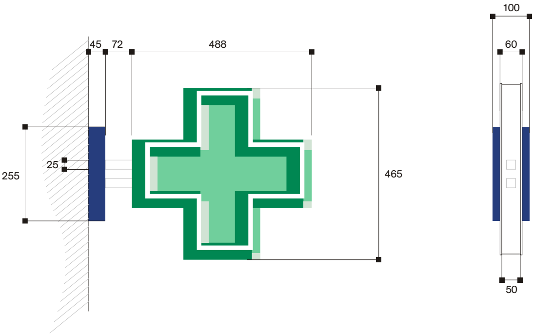
Projecting Sign Detail Scale: 1:10@A3
