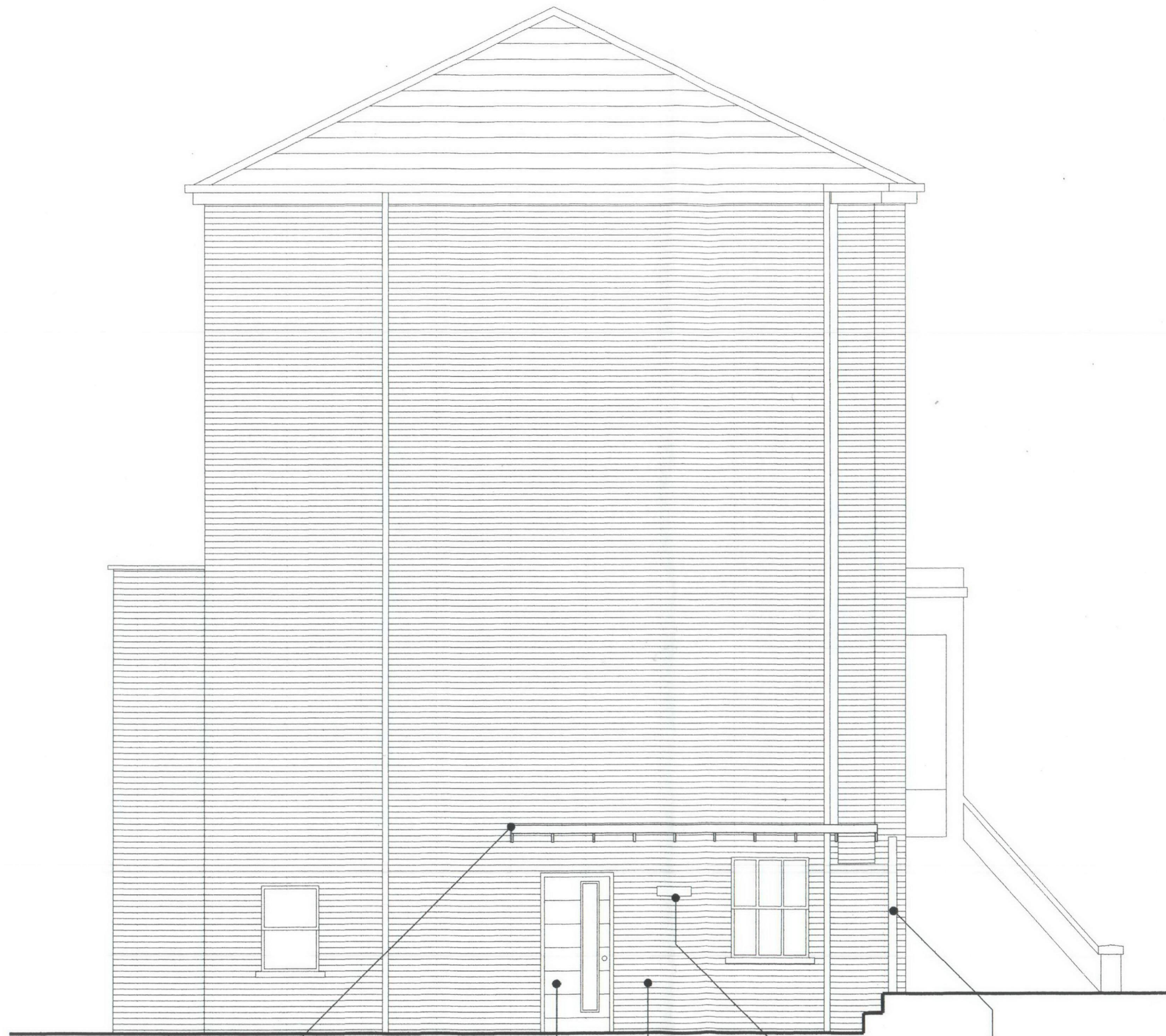
SIDE ELEVATION (PROPOSED)
