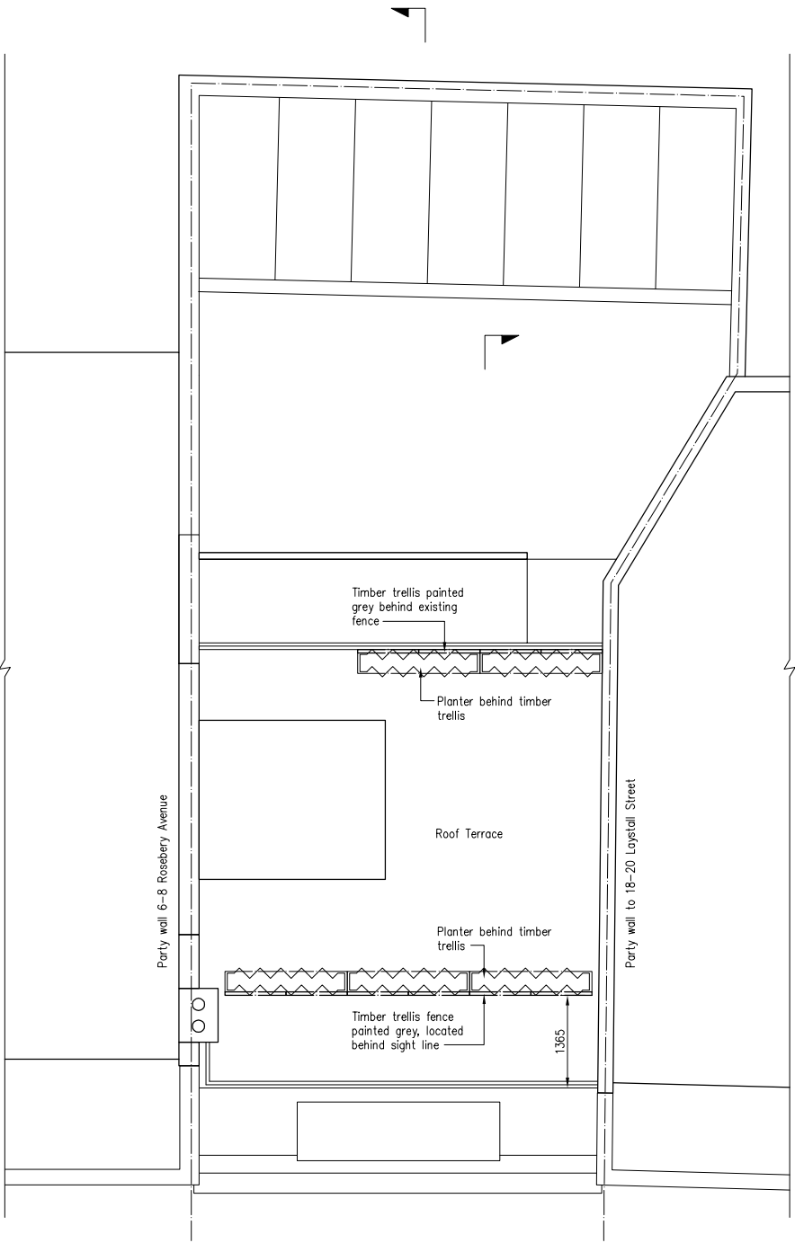
Roof Plan
