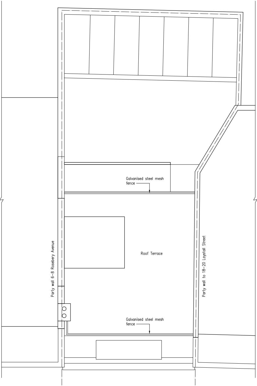
Roof Plan
