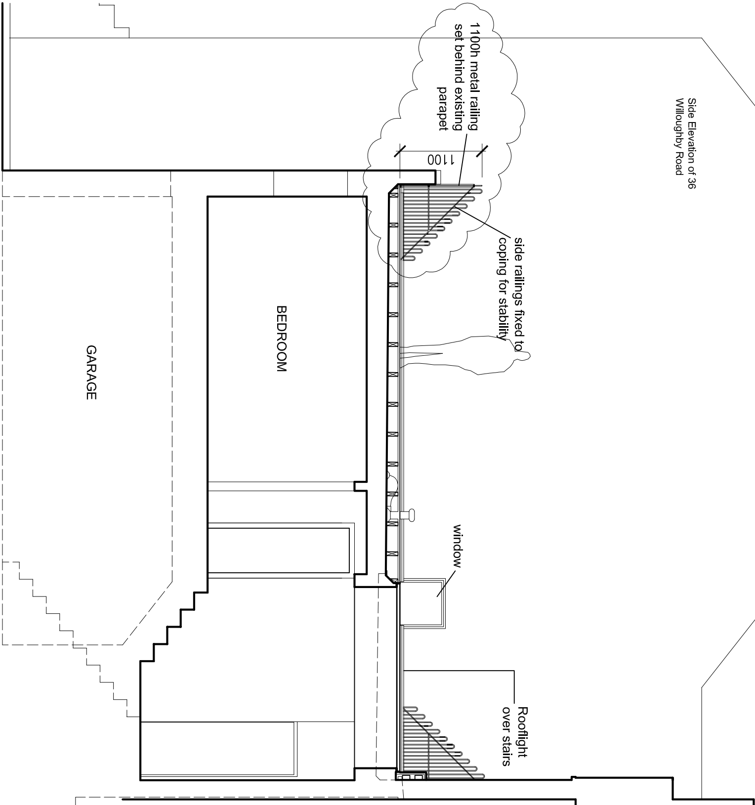
SECTION BB (through Rooflight in terrace)
