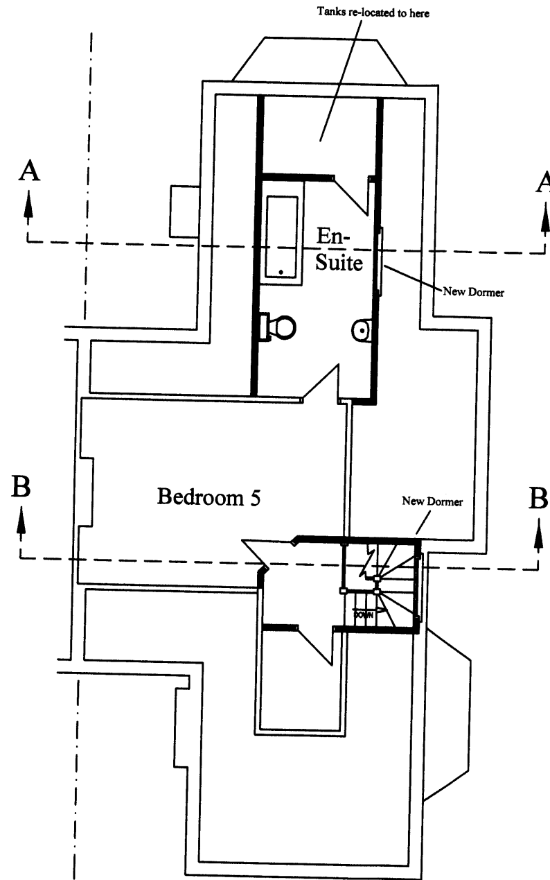
PROPOSED LOFT FLOOR
