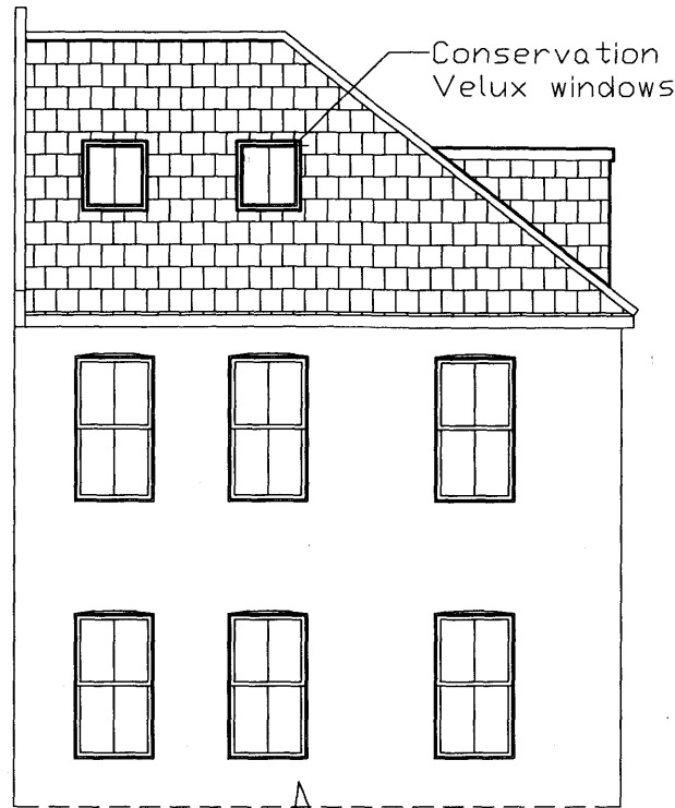
REAR ELEVATION
