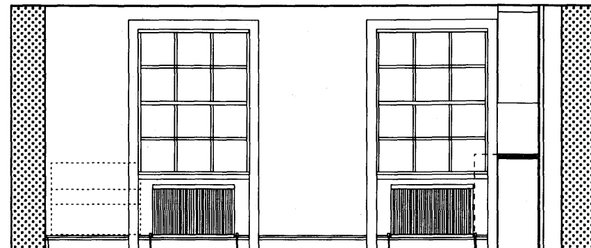
ELEVATION 4.1
