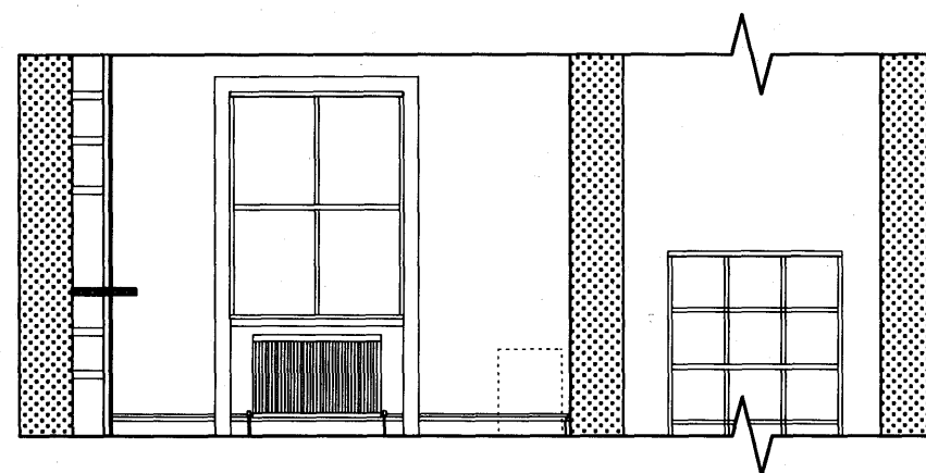
ELEVATION 4.3
