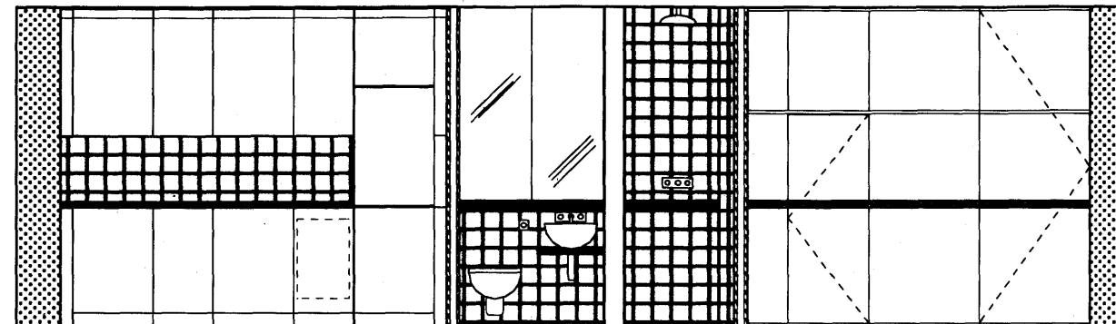
ELEVATION 4.2
