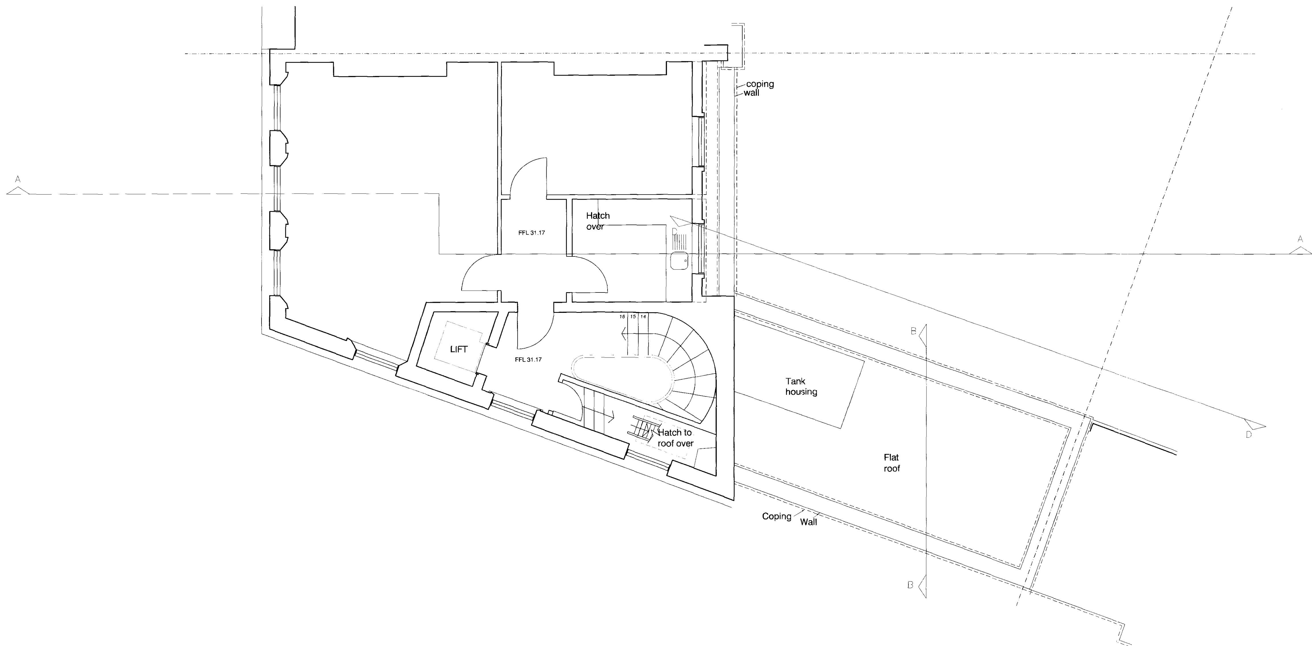
PL_E_005 EXISTING THIRD FLOOR PLAN 01 SCALE 1:50@A1
