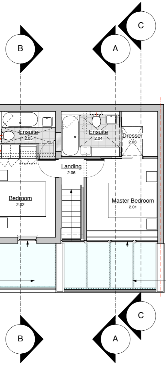
1 Second Floor Plan - Proposed Scale: 1:100 @ A3
