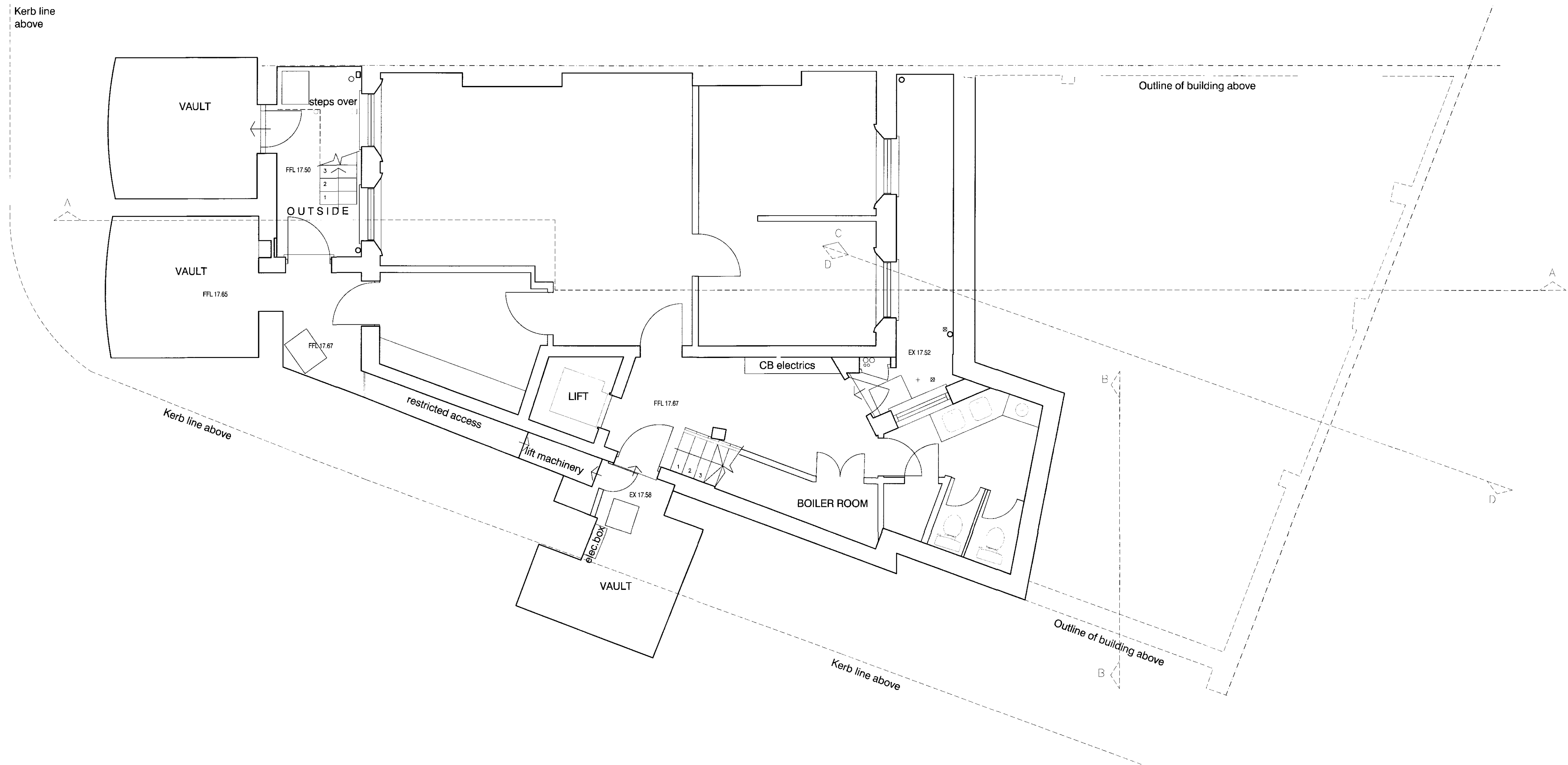
PL_E_001 EXISTING BASEMENT PLAN 01 SCALE 1:50@A1
