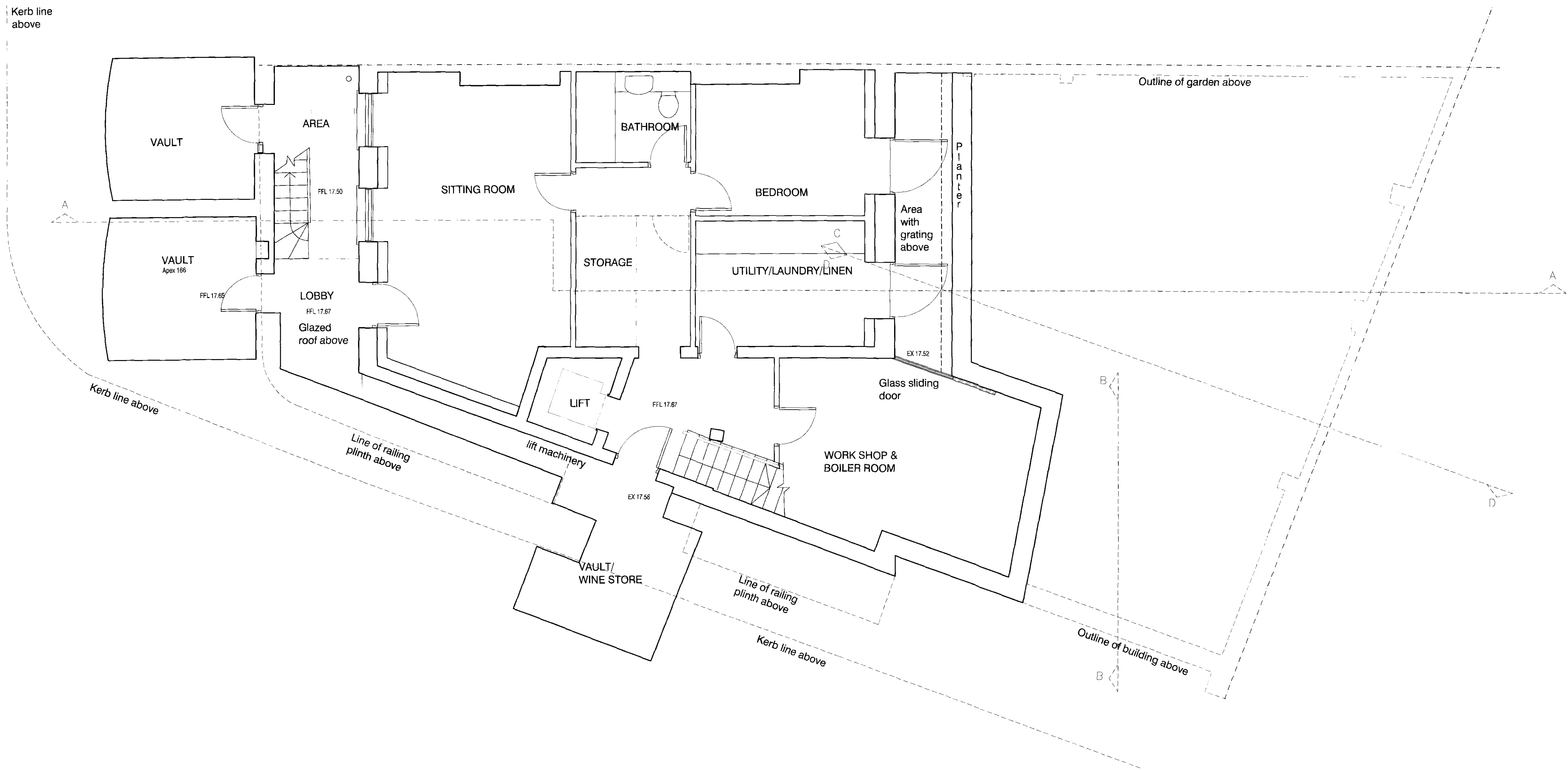
PL_P_001 PROPOSED BASEMENT PLAN 01 SCALE 1: 50@A1
