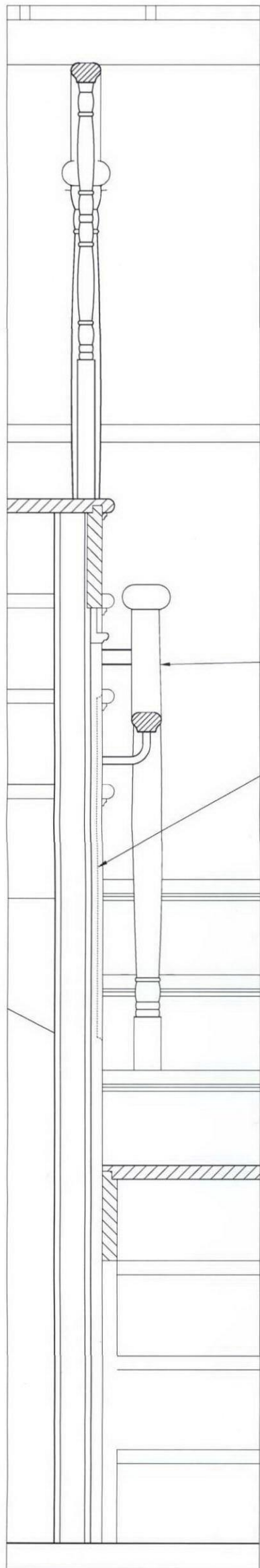
DETAIL C
