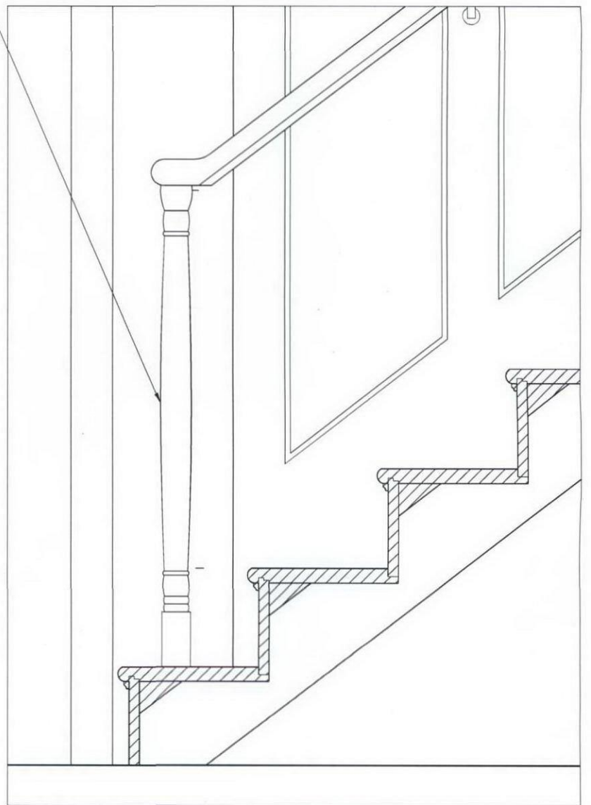
DETAIL A
