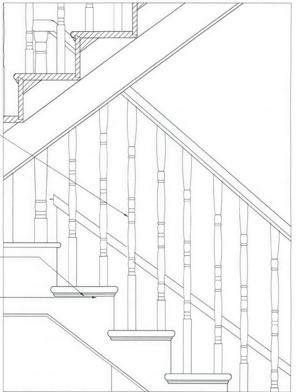
DETAIL D
