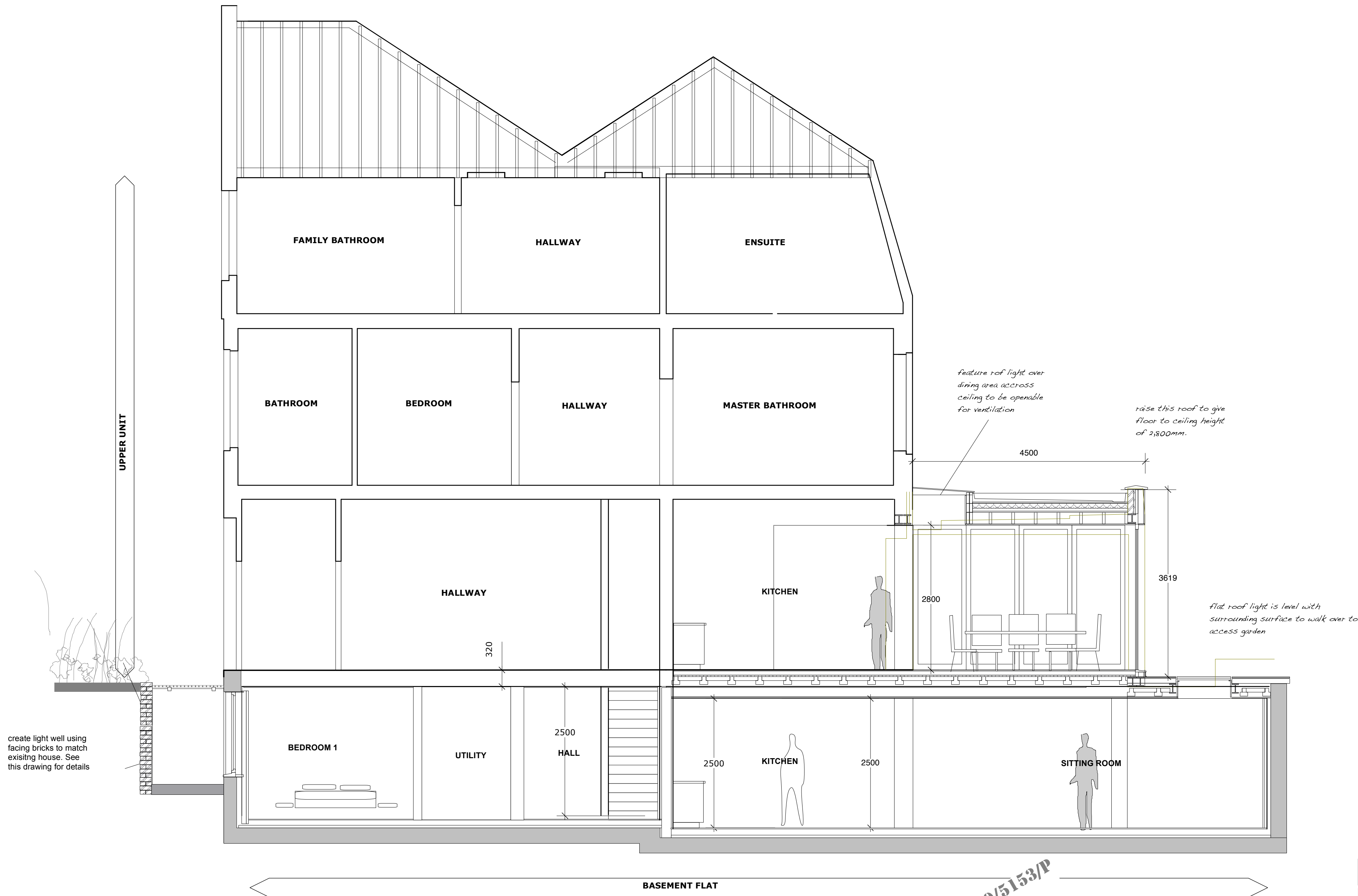
Proposed Section A-A
