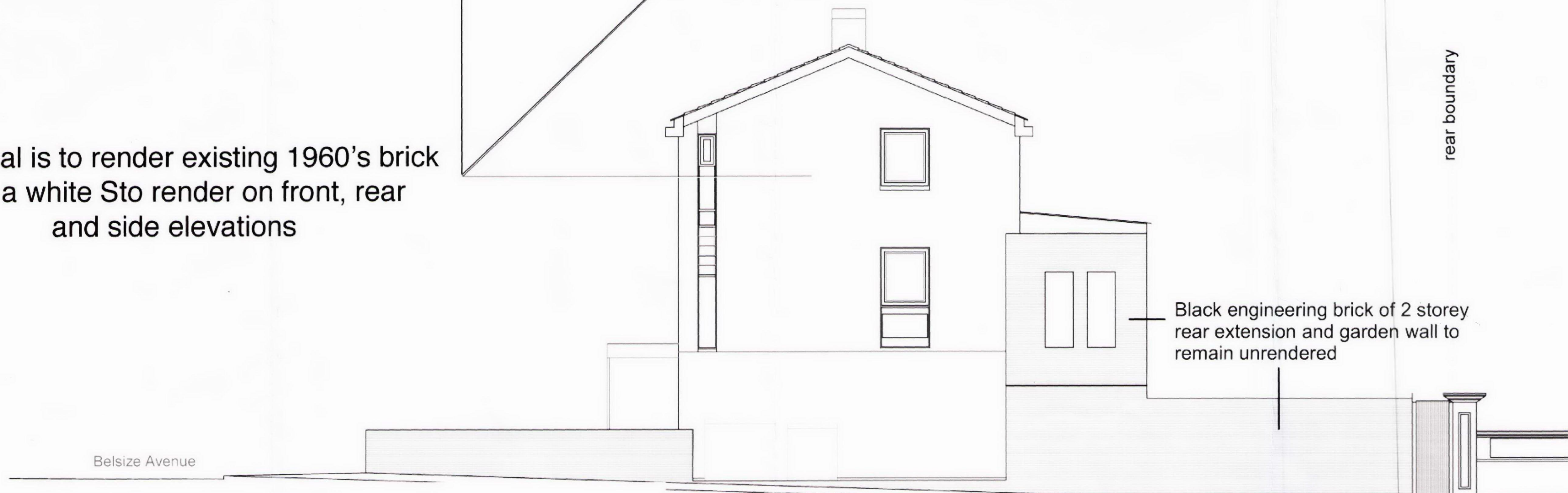
PROPOSED SIDE ELEVATION FROM BELSIZE PARK GARDENS
