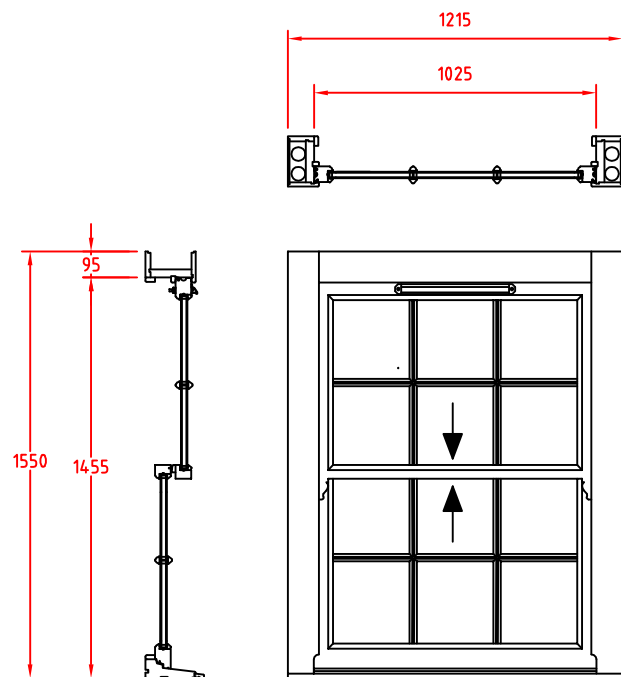
Sash & Case Mk2 Window Ref. WT11-29
