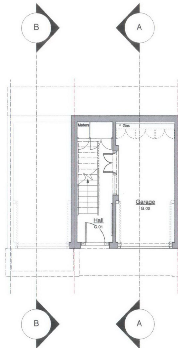
1 Ground Floor Plan - Existing Scale: 1:100 @ A3
