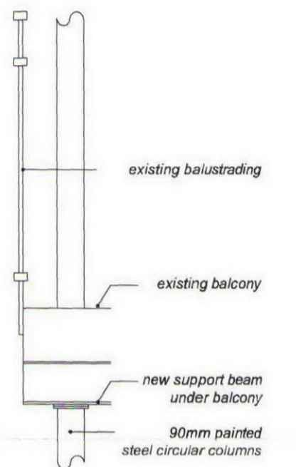
Section through balcony 1:20
