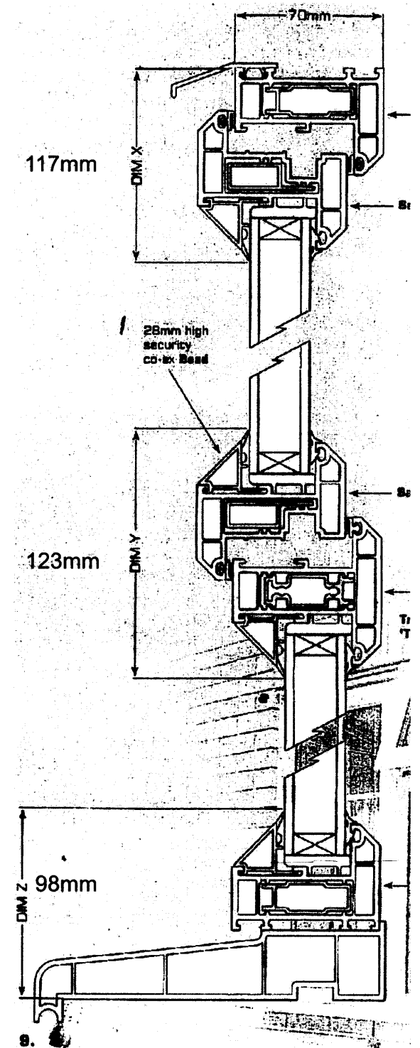
Typical window section NTS
