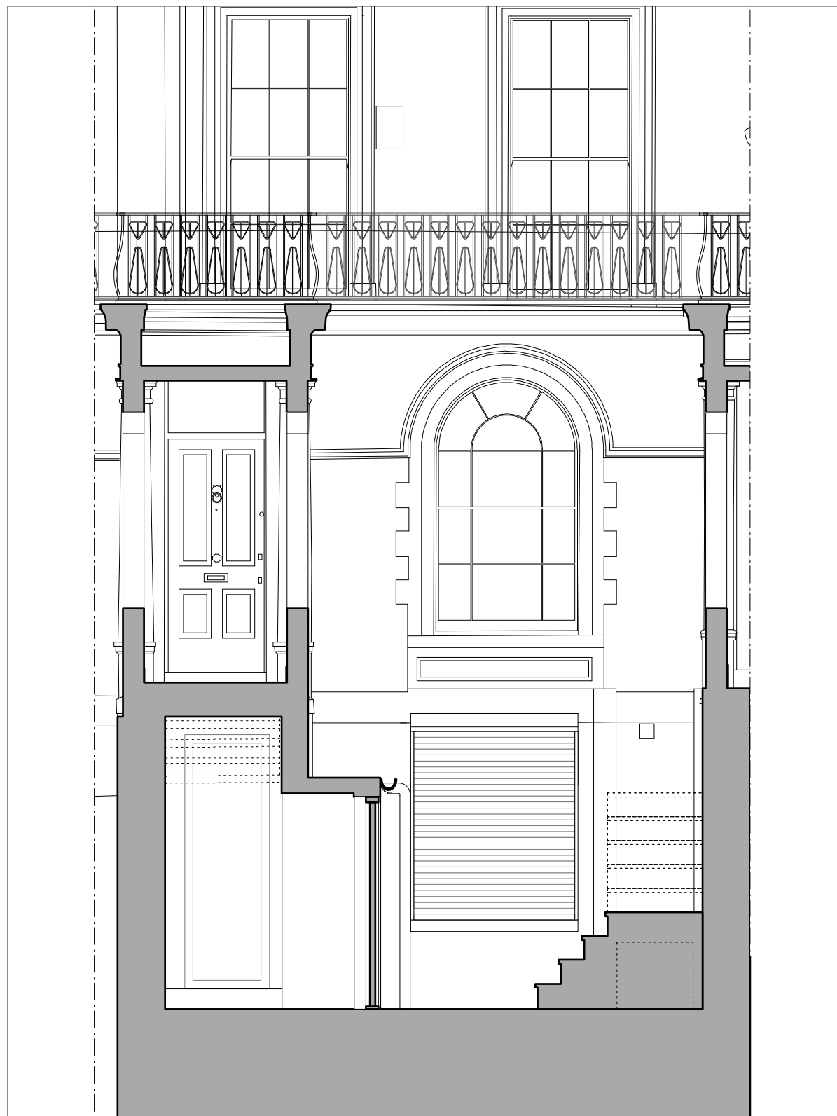
Lightwell Section C-C
