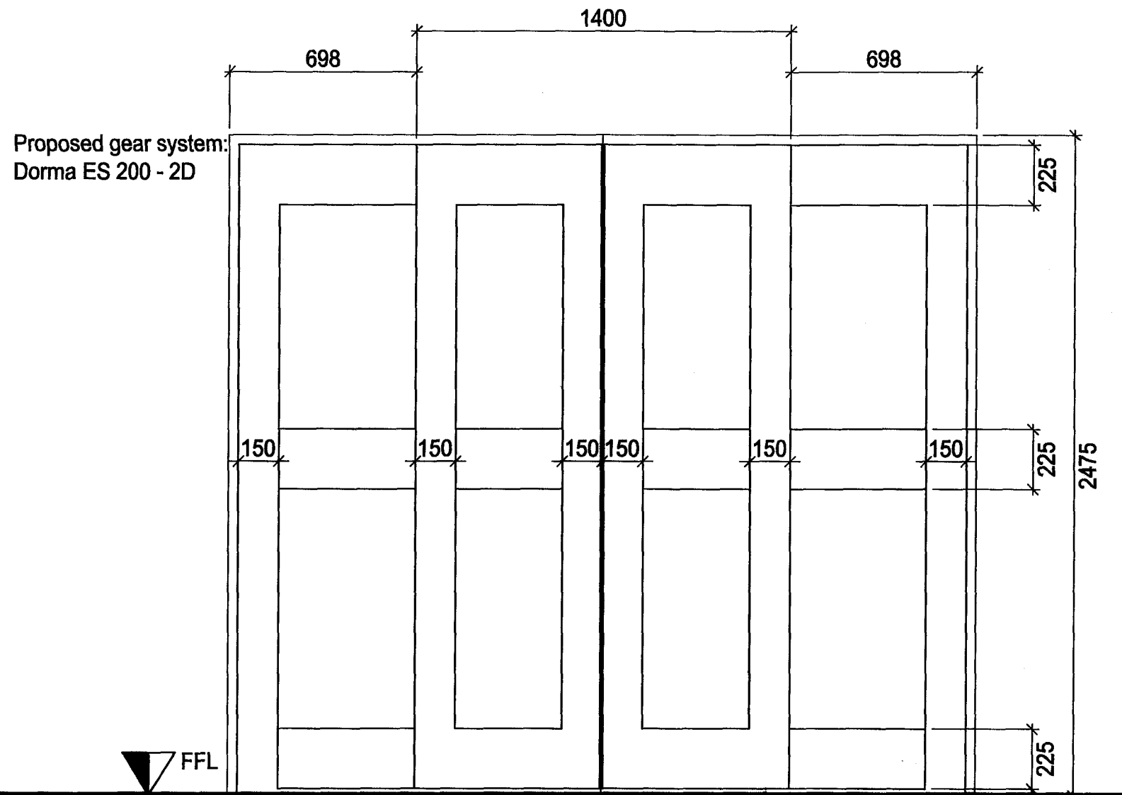
Entrance Door - Elevation
