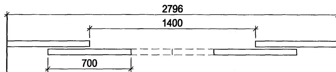
Entrance Door - Plan
