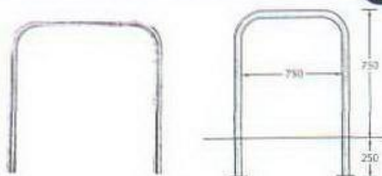
SHEFFIELD CYCLE STAND
