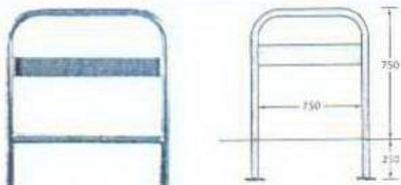
SHEFFIELD CYCLE STAND WITH SIGN STRIP & TAPPING BAR
