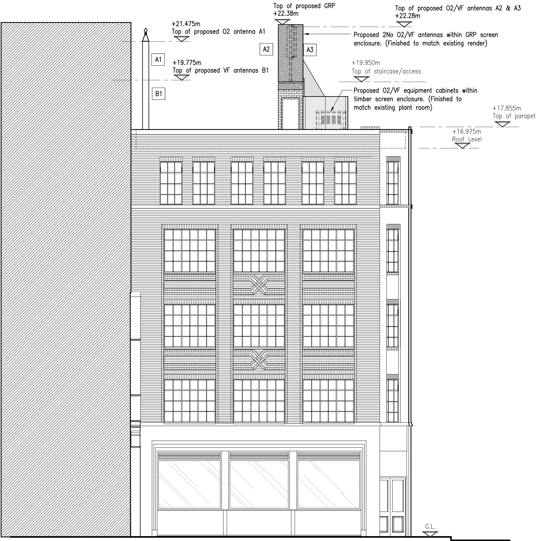
PROPOSED SITE ELEVATION (1:100)
