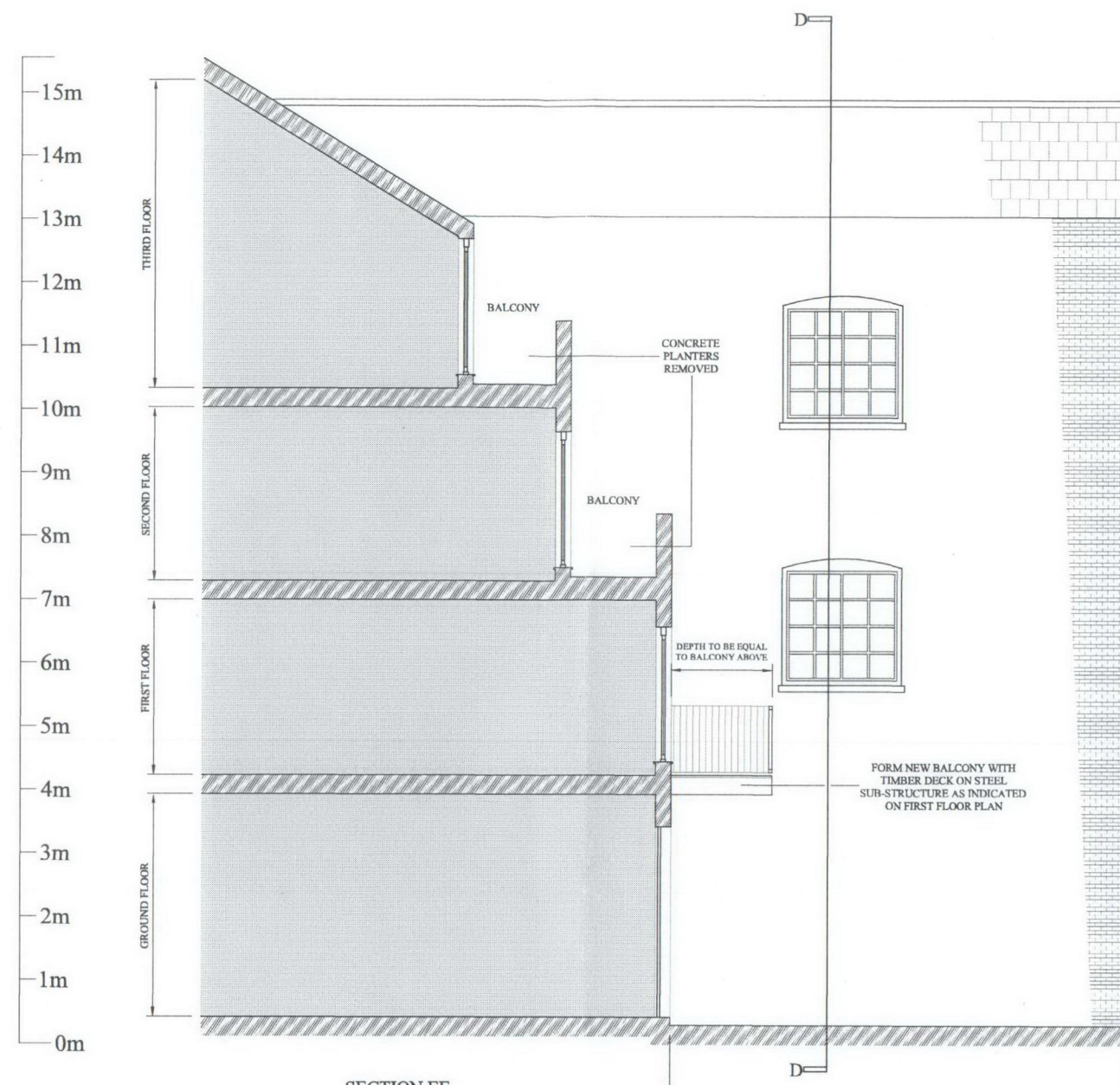
SECTION EE AS PROPOSED RESIDENTIAL
