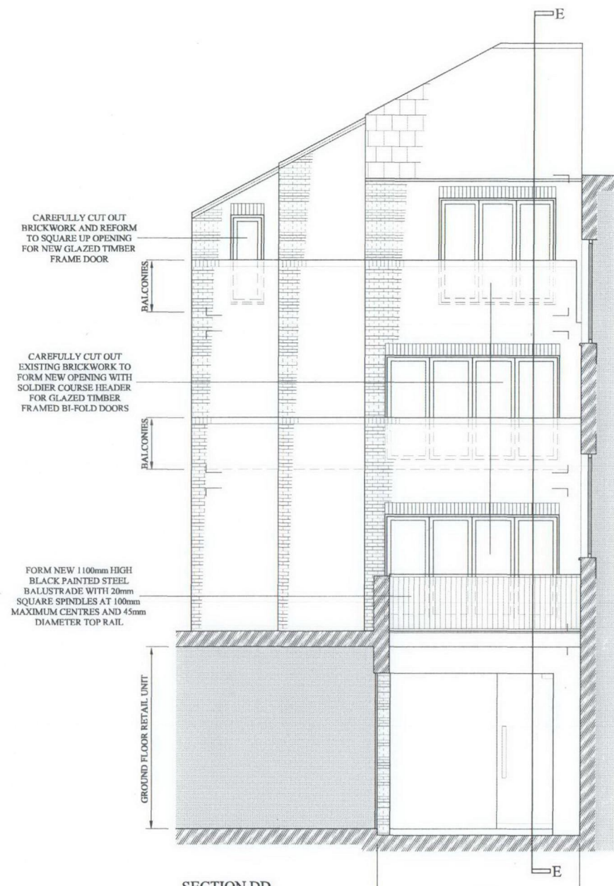
SECTION DD AS PROPOSED RESIDENTIAL
