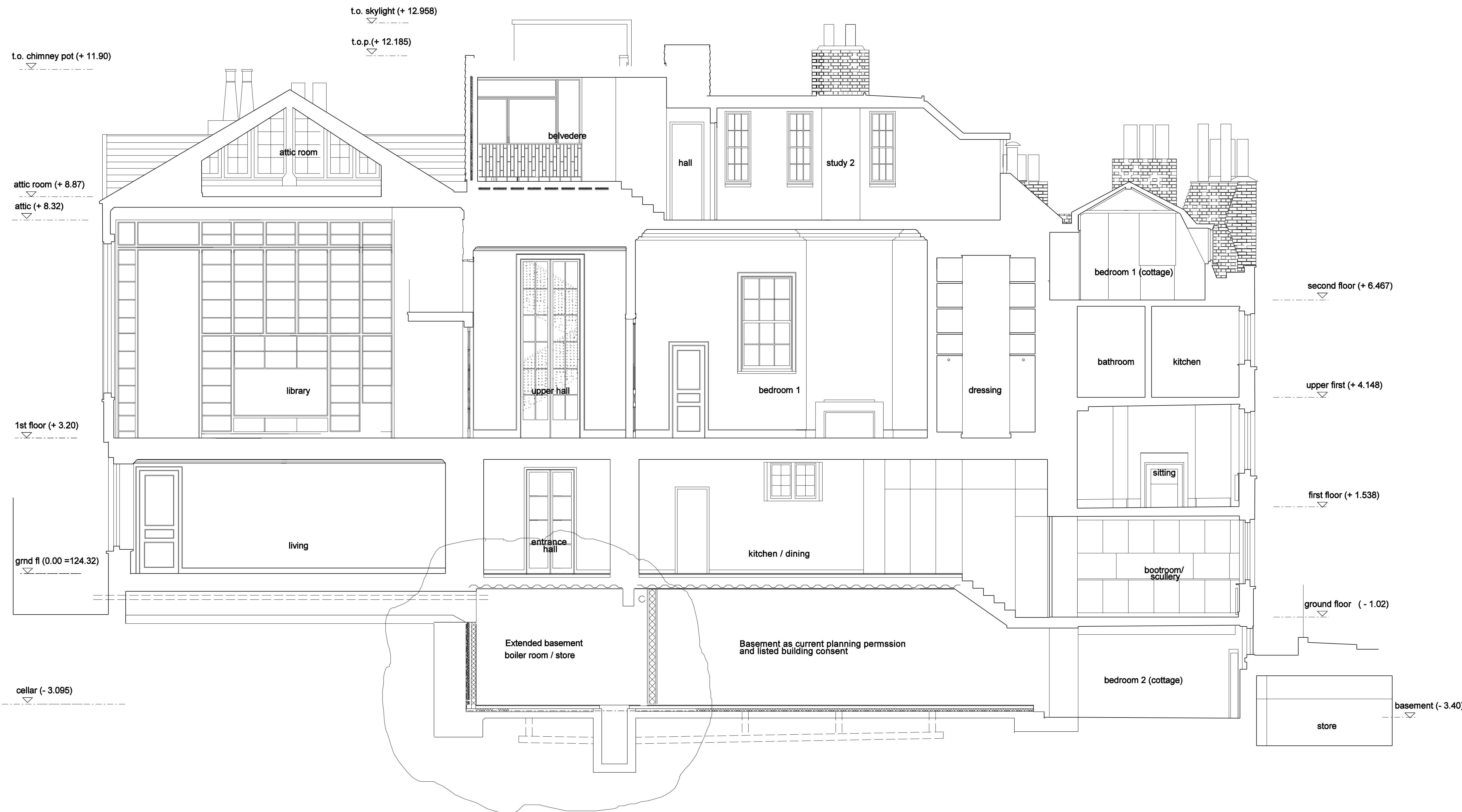
Section GG - Proposed extended basement
