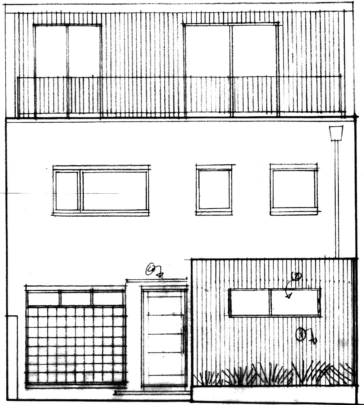
FRONT ELEVATION
