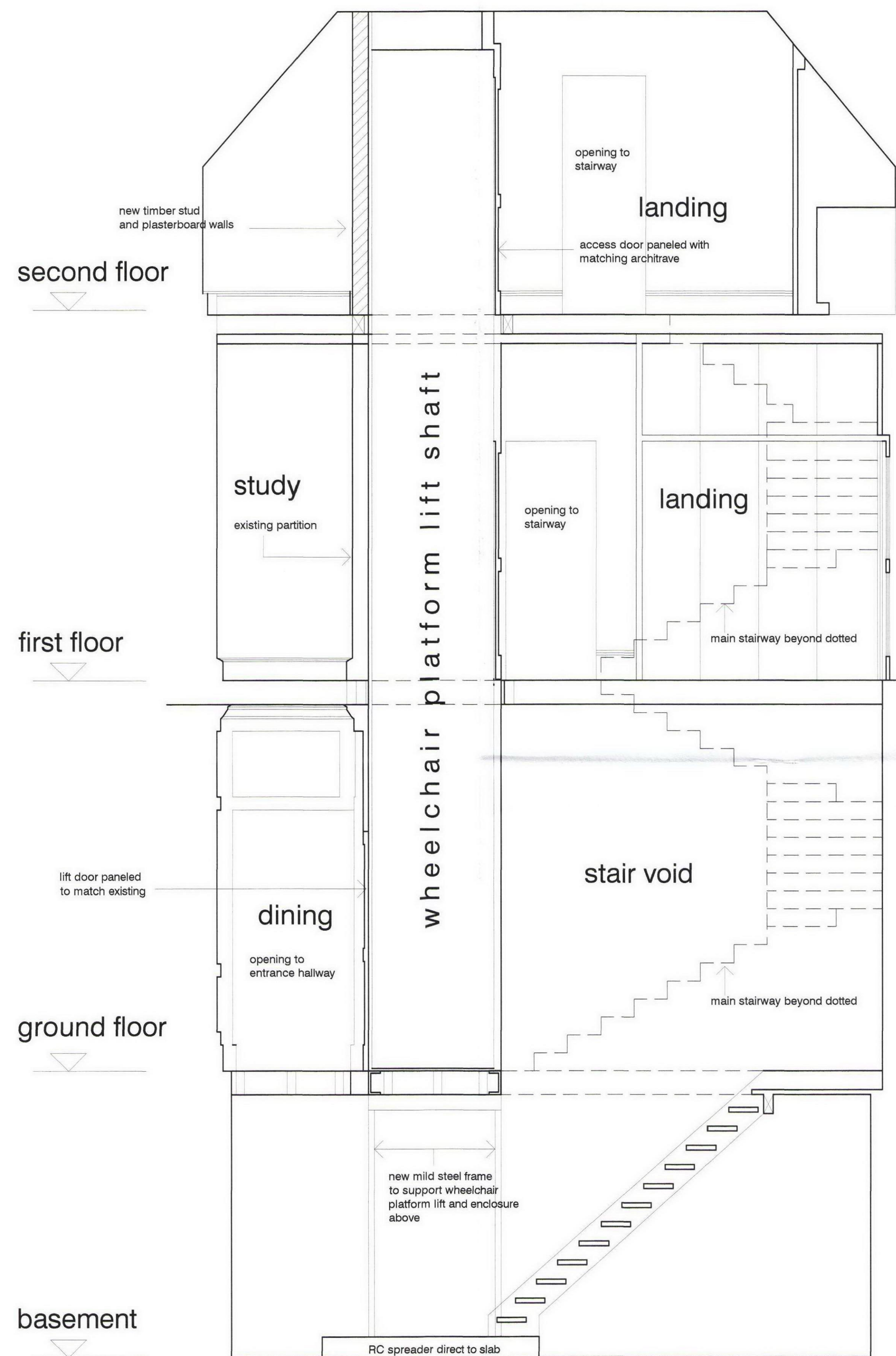
section AA proposed
