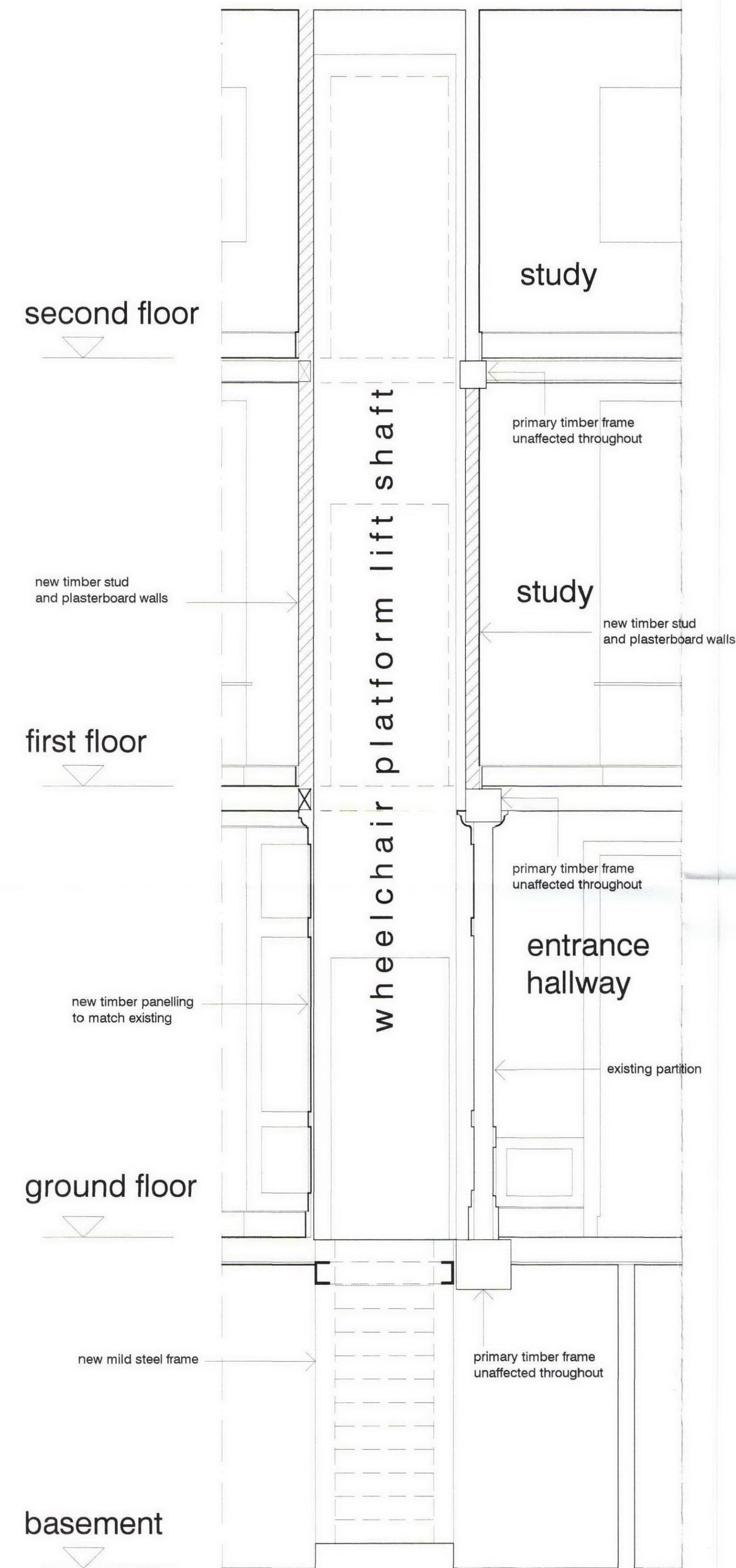
section BB proposed
