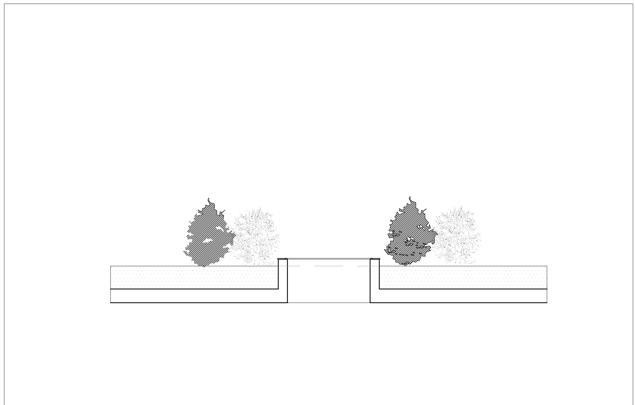
Typical Skylight detail to include for 150mm upstand above soil and stone capped perimeter to glass.
