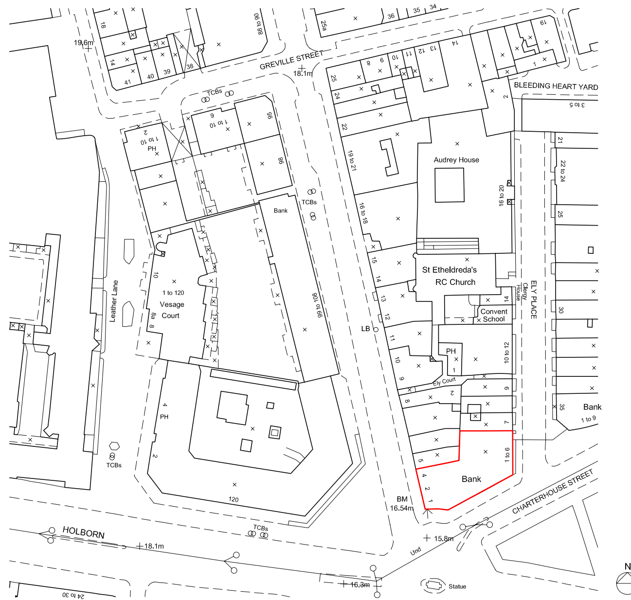
LOCATION PLAN 1:1250
