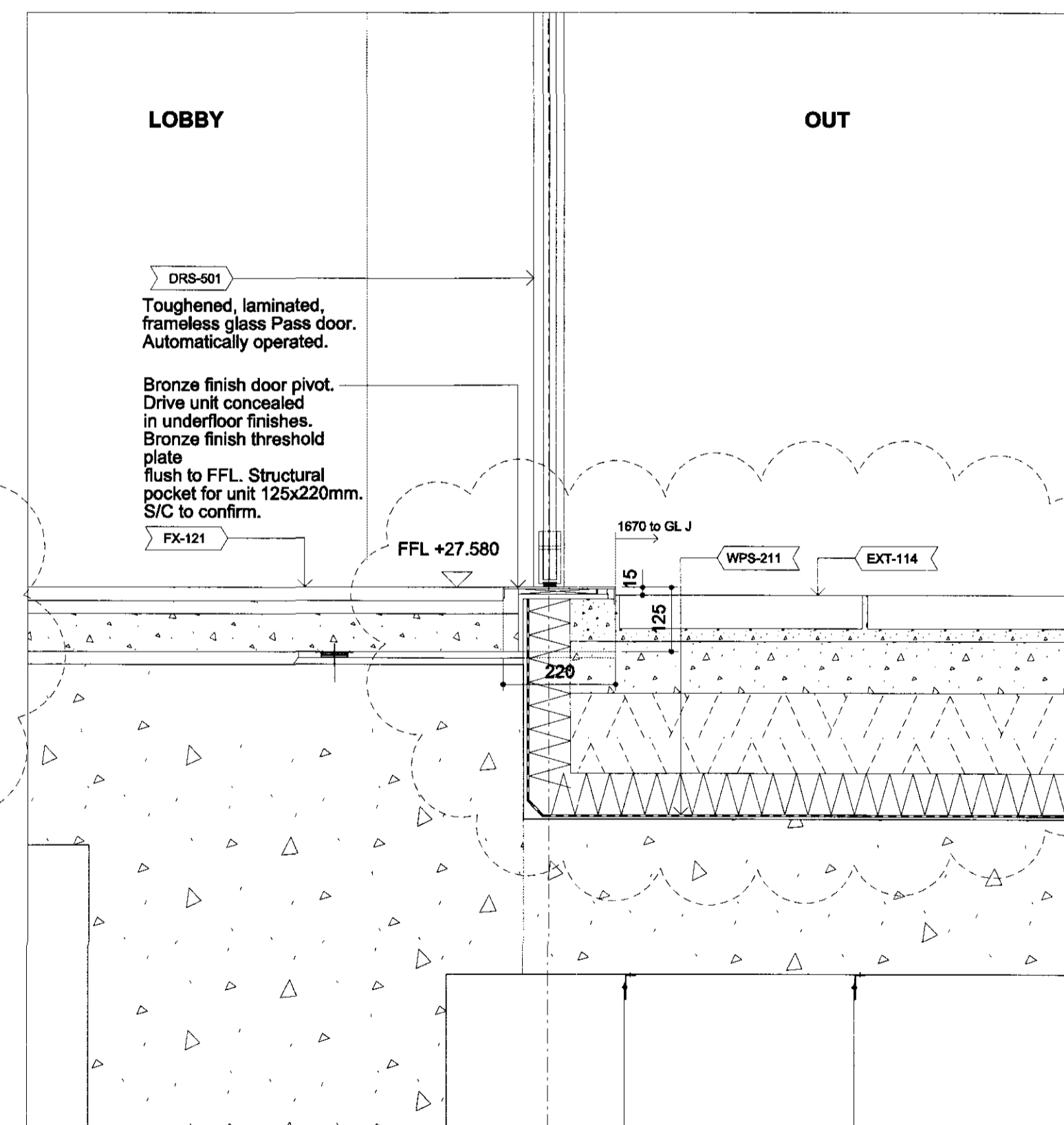
Detail 03 - Cross-section through Entrance Pass door.
