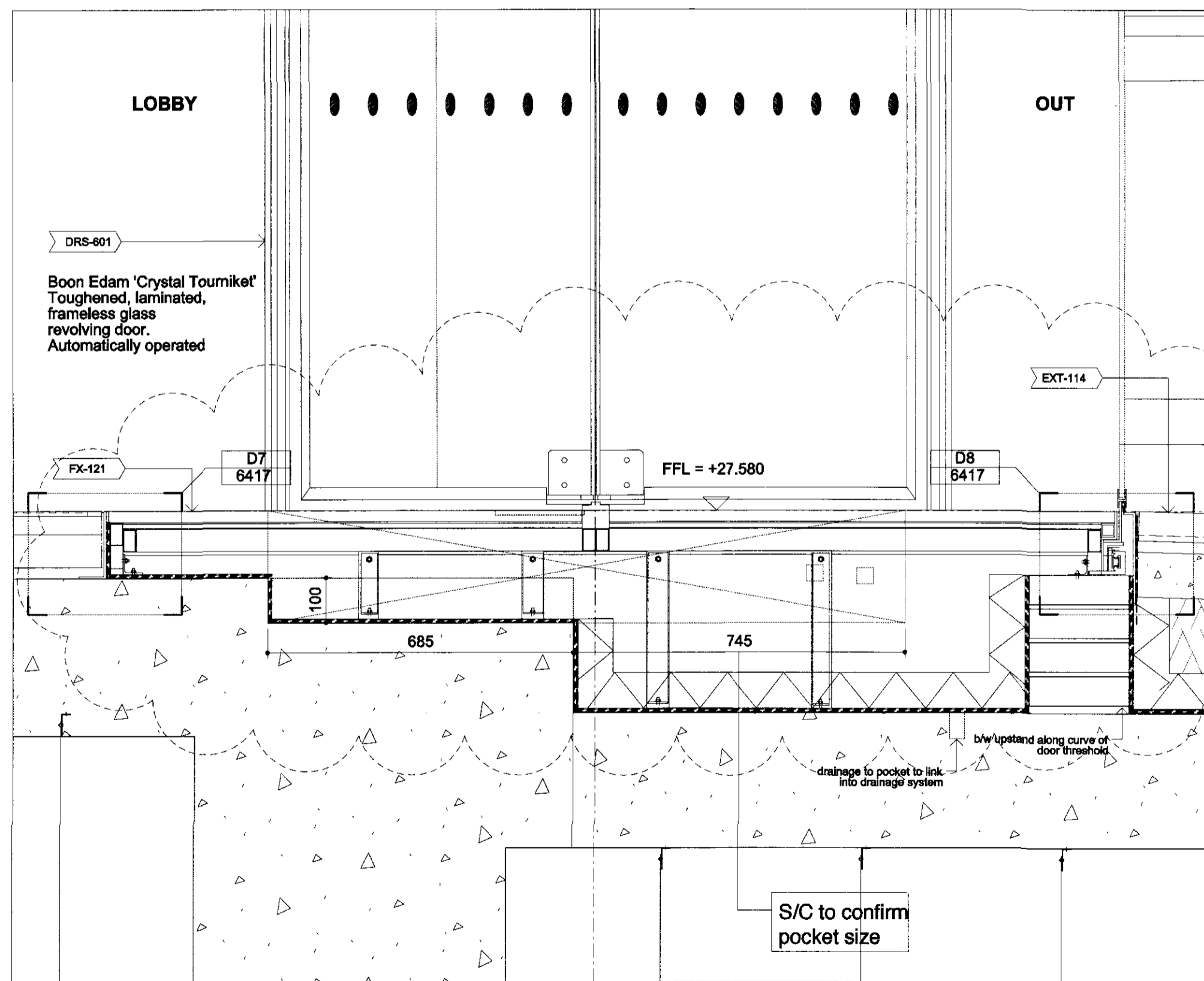
Detail 02 - Cross-section through Entrance Revolving door.
