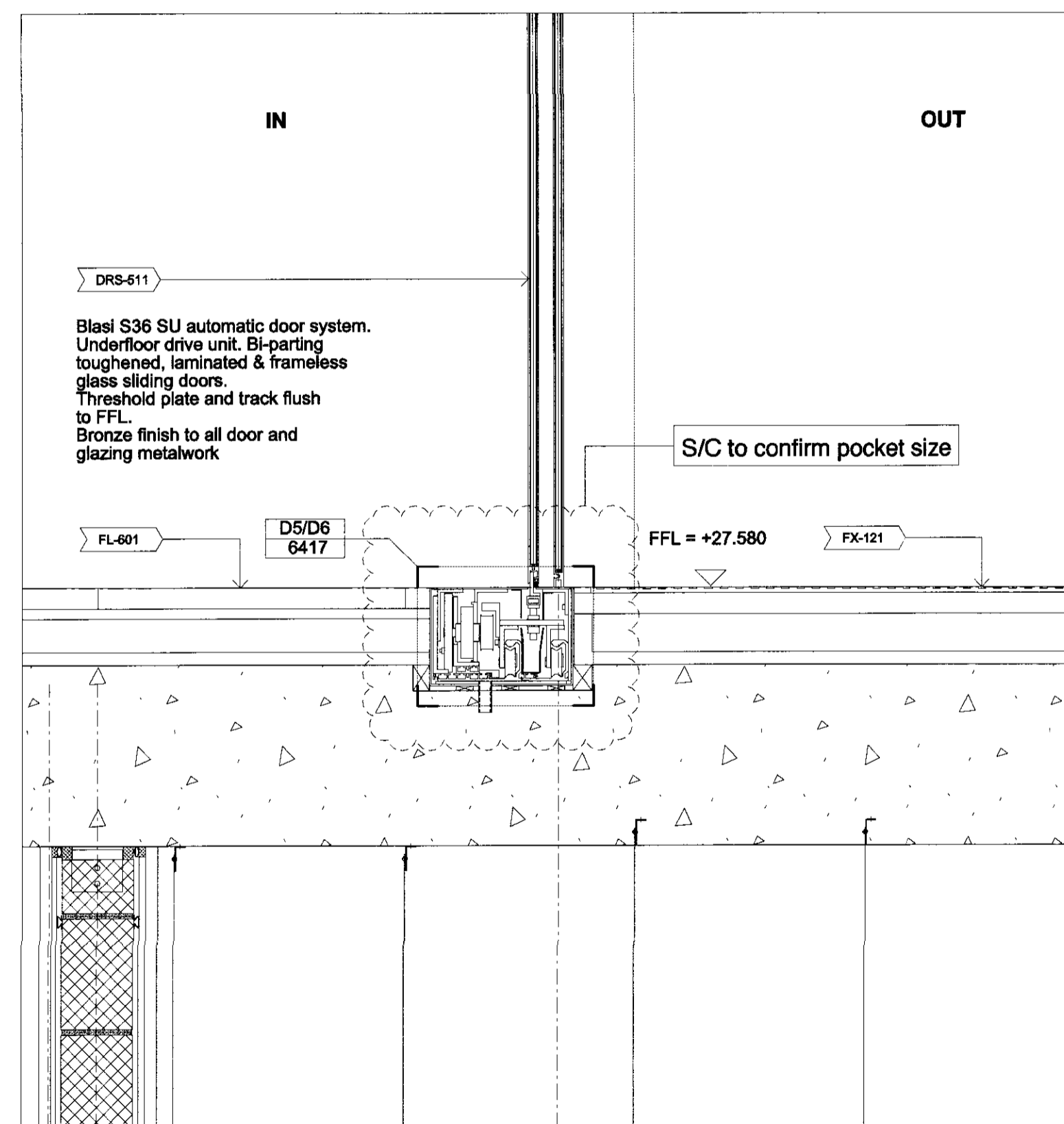
Detail 01 - Cross-section through Draught Lobby Sliding door
