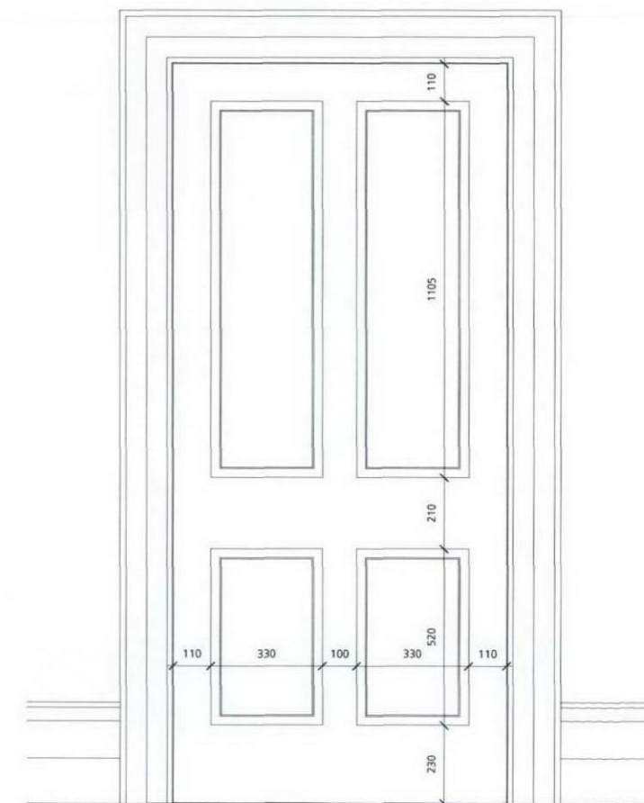
ELEVATION 1:10
