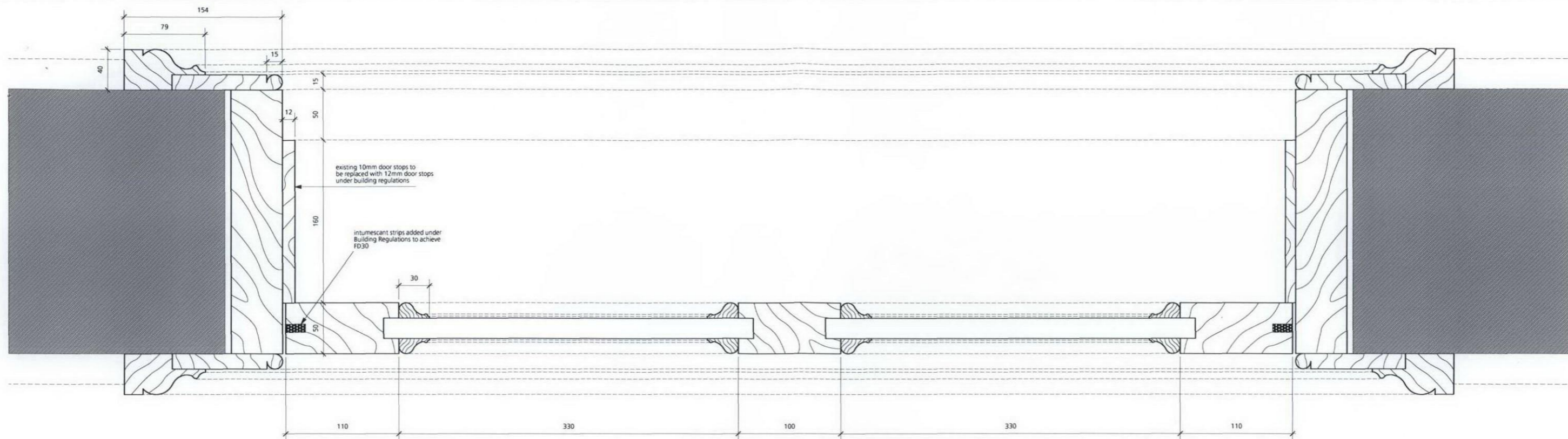
ORIGINAL DOOR WITH UPGRADED DOORSTOPS 1:2
