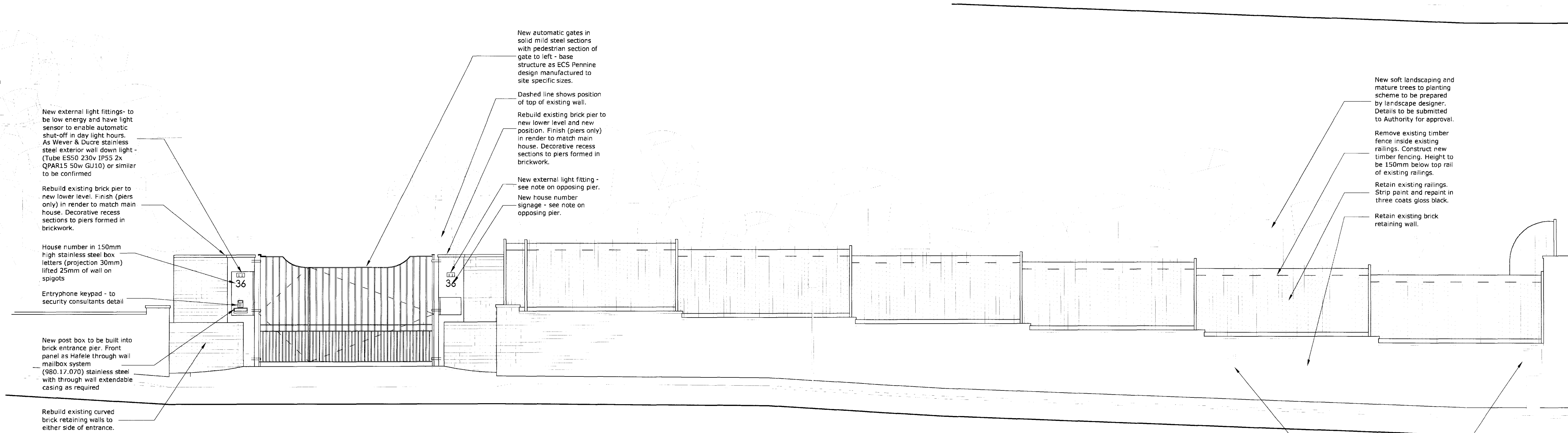
Proposed Street Elevation 1:50 - 19 March 2010
