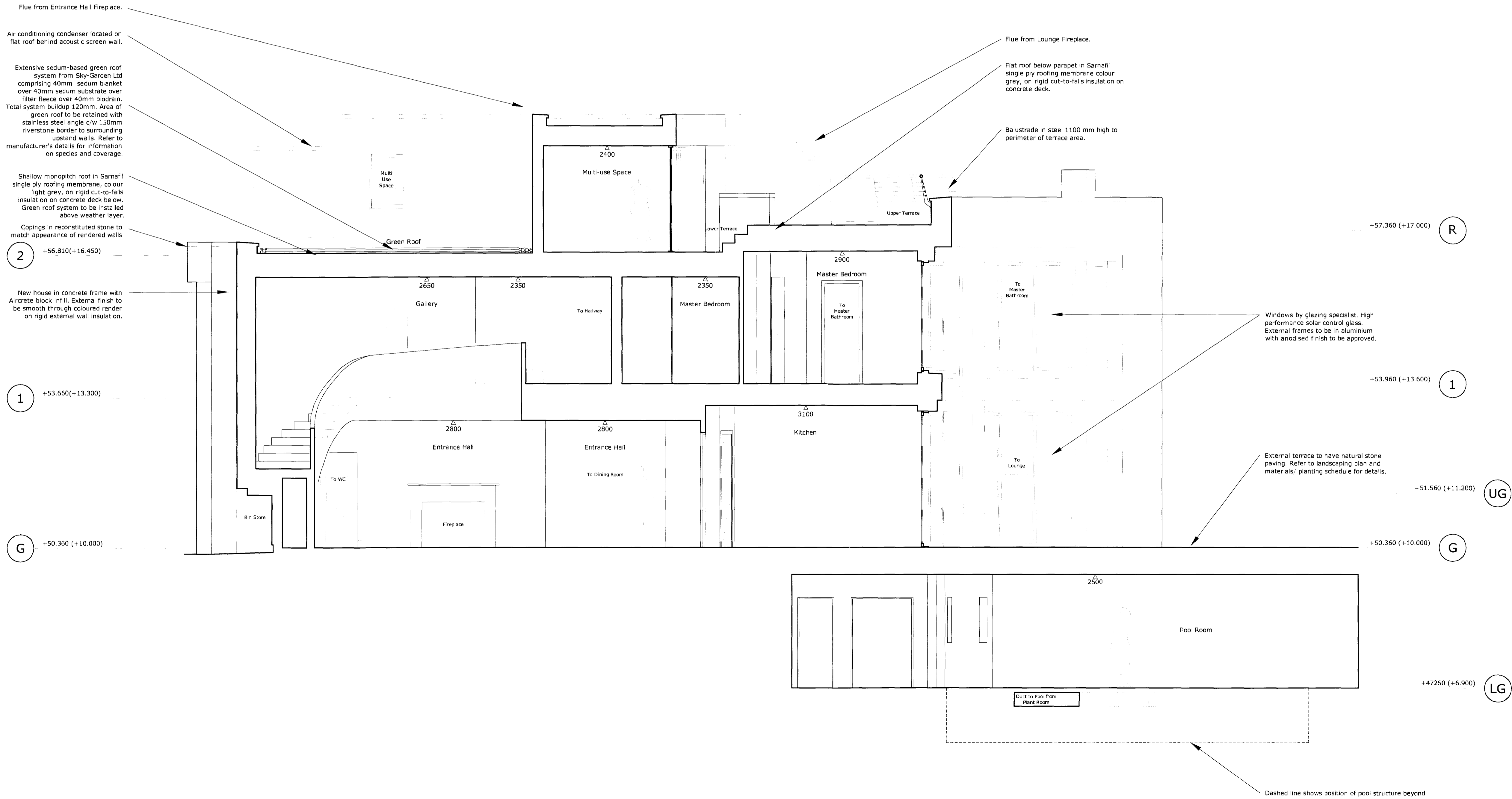
Proposed Section A-A 1:50 - 15 March 2010
