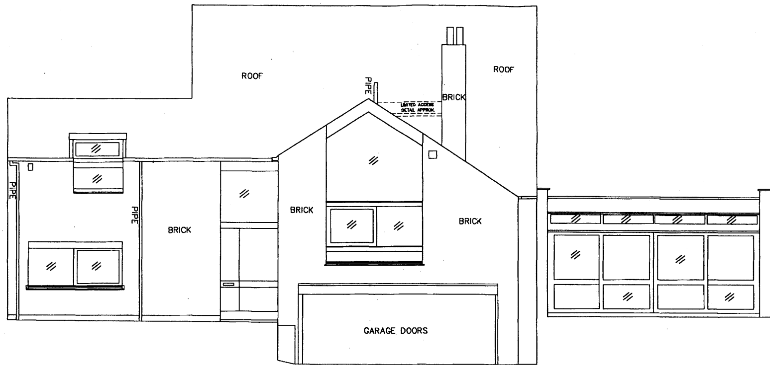
WEST ELEVATION
