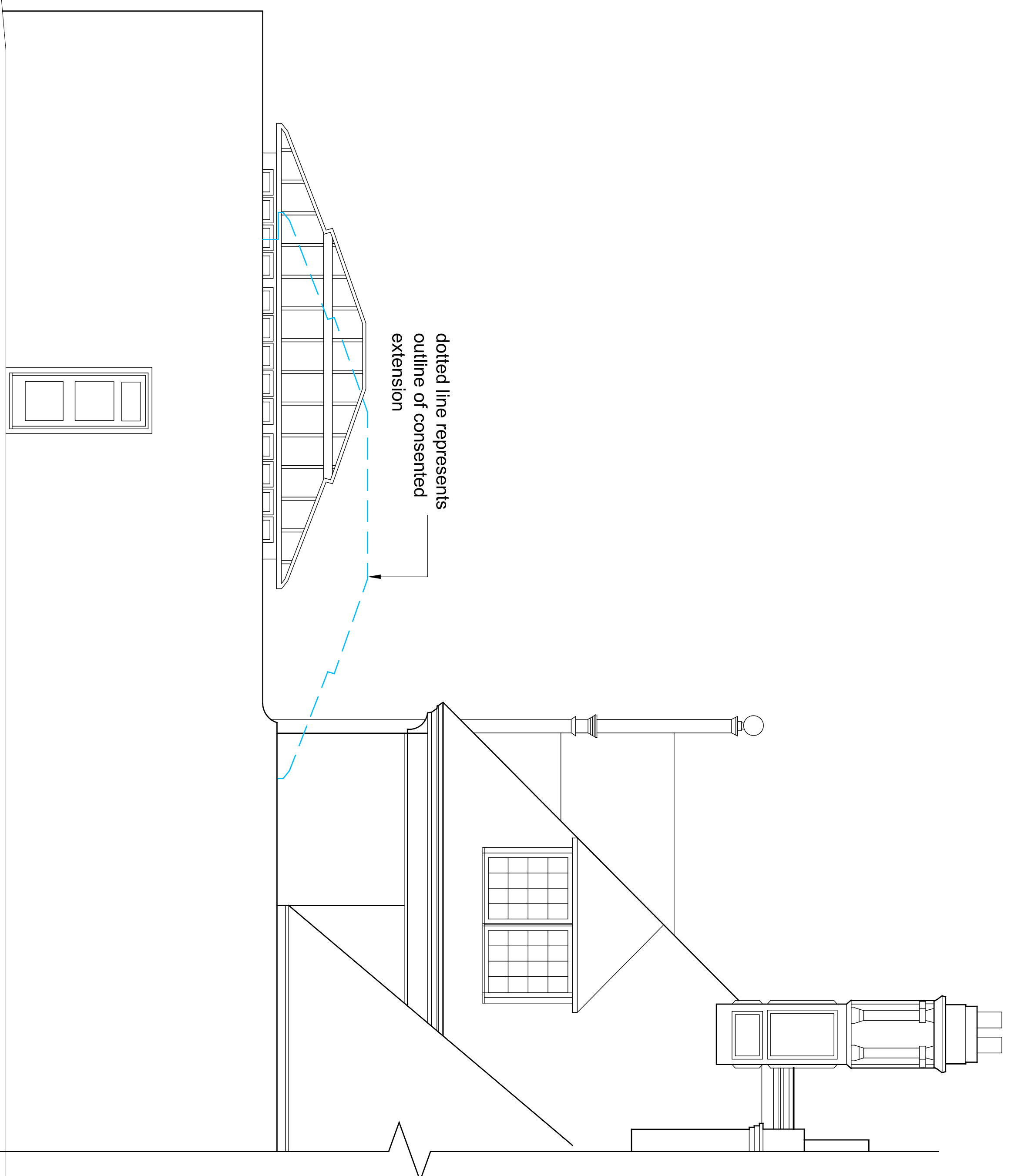
PROPOSED EAST ELEVATION
