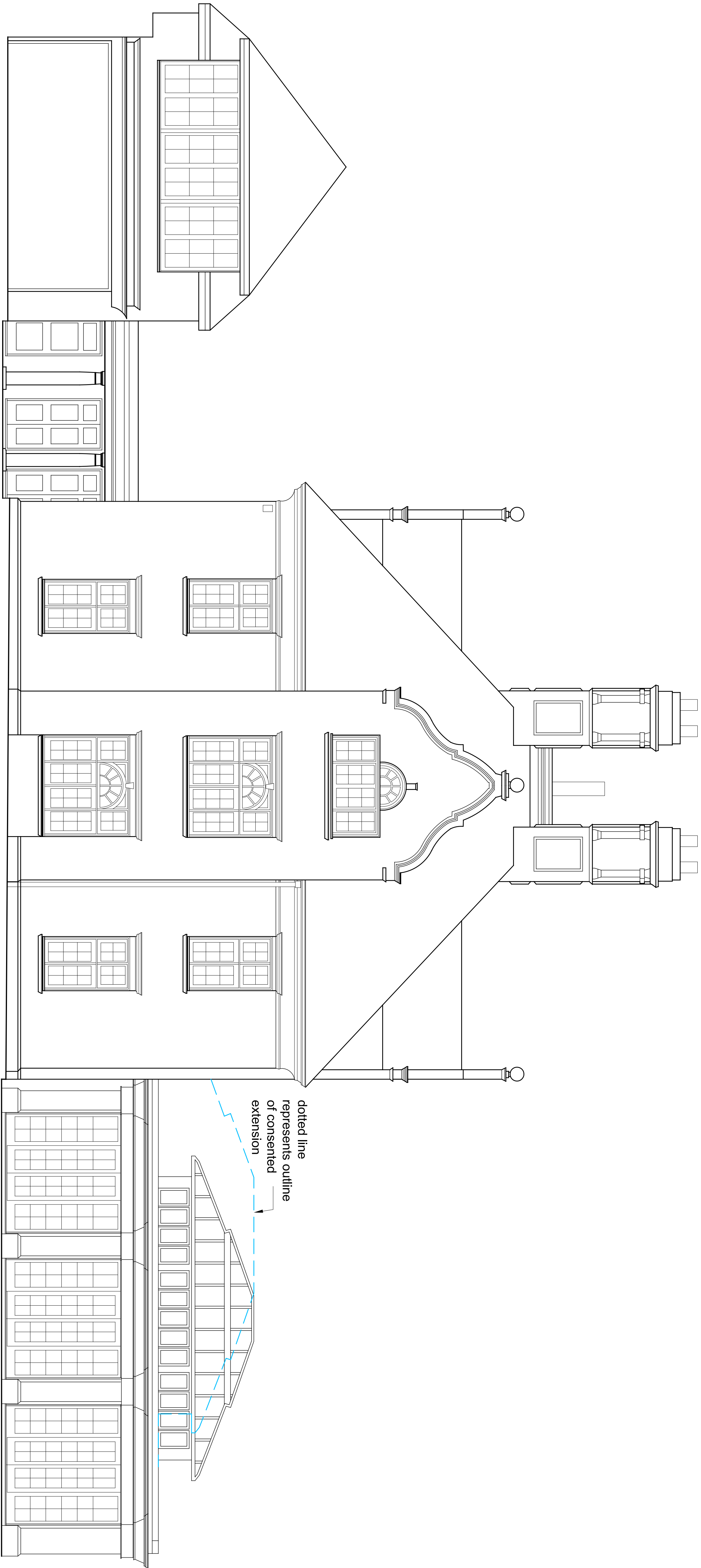
PROPOSED WEST ELEVATION
