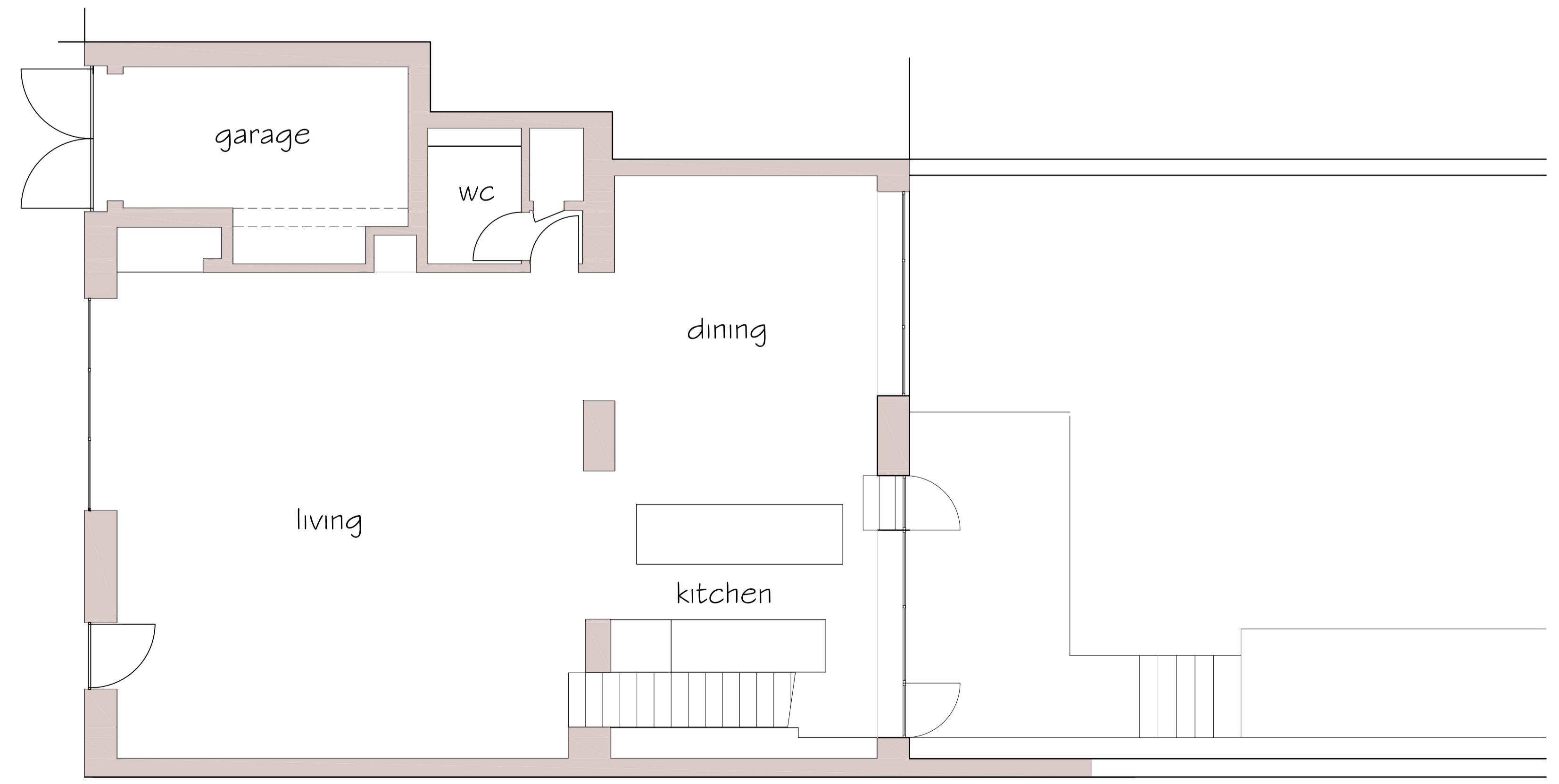
Ground Floor
