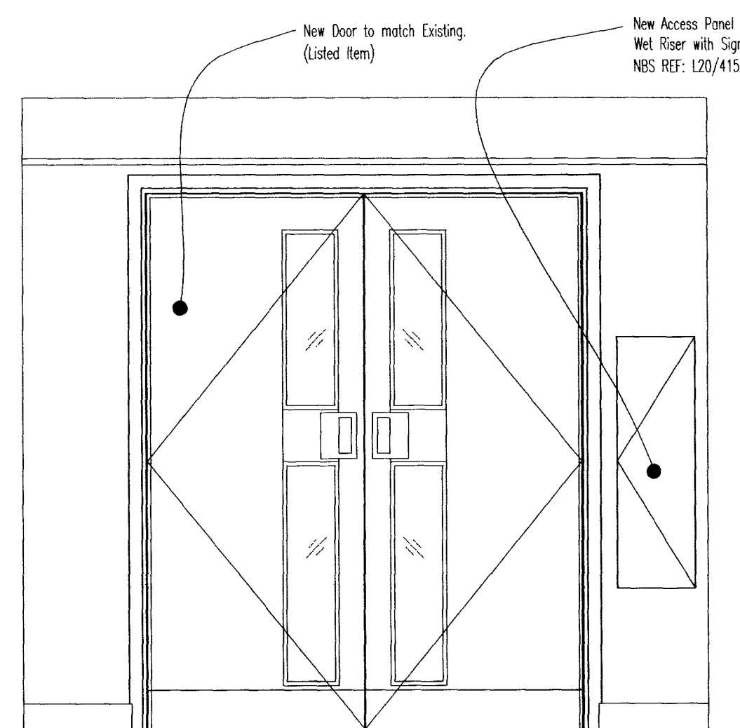
Elevation C-C Proposed
