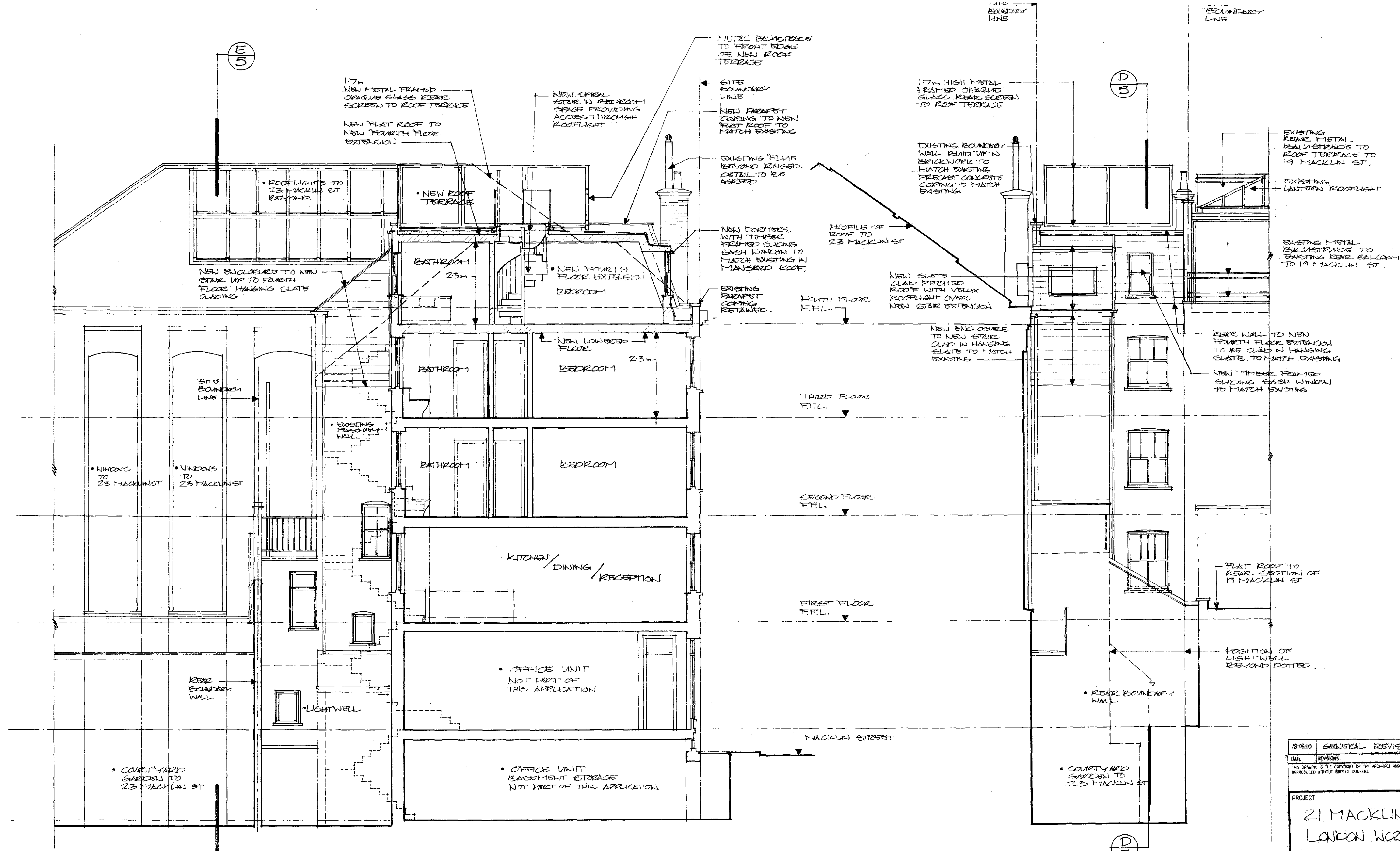
PROPOSED SECTION (D 5)
