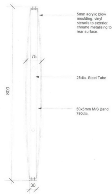
1 1:10 Section through projecting sign 446
