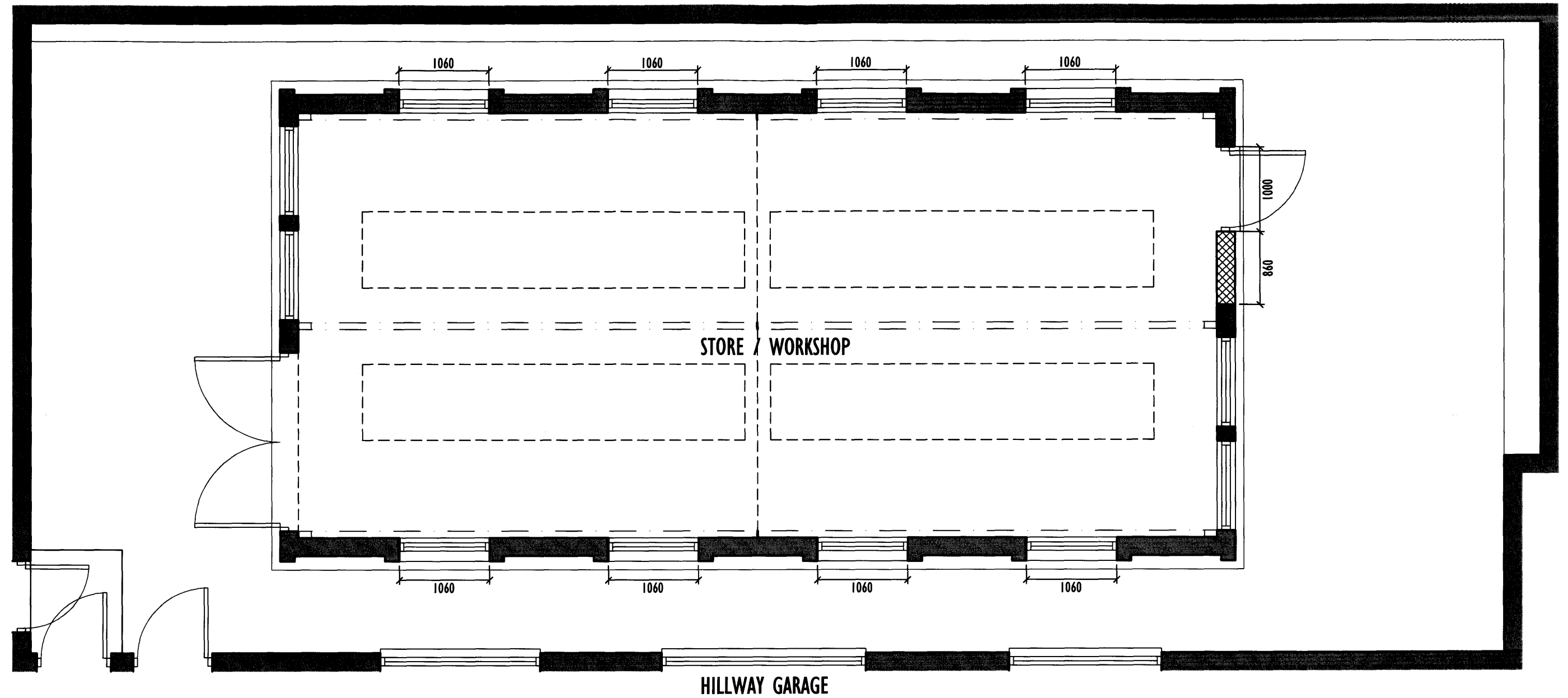
PROPOSED FLOOR PLAN
