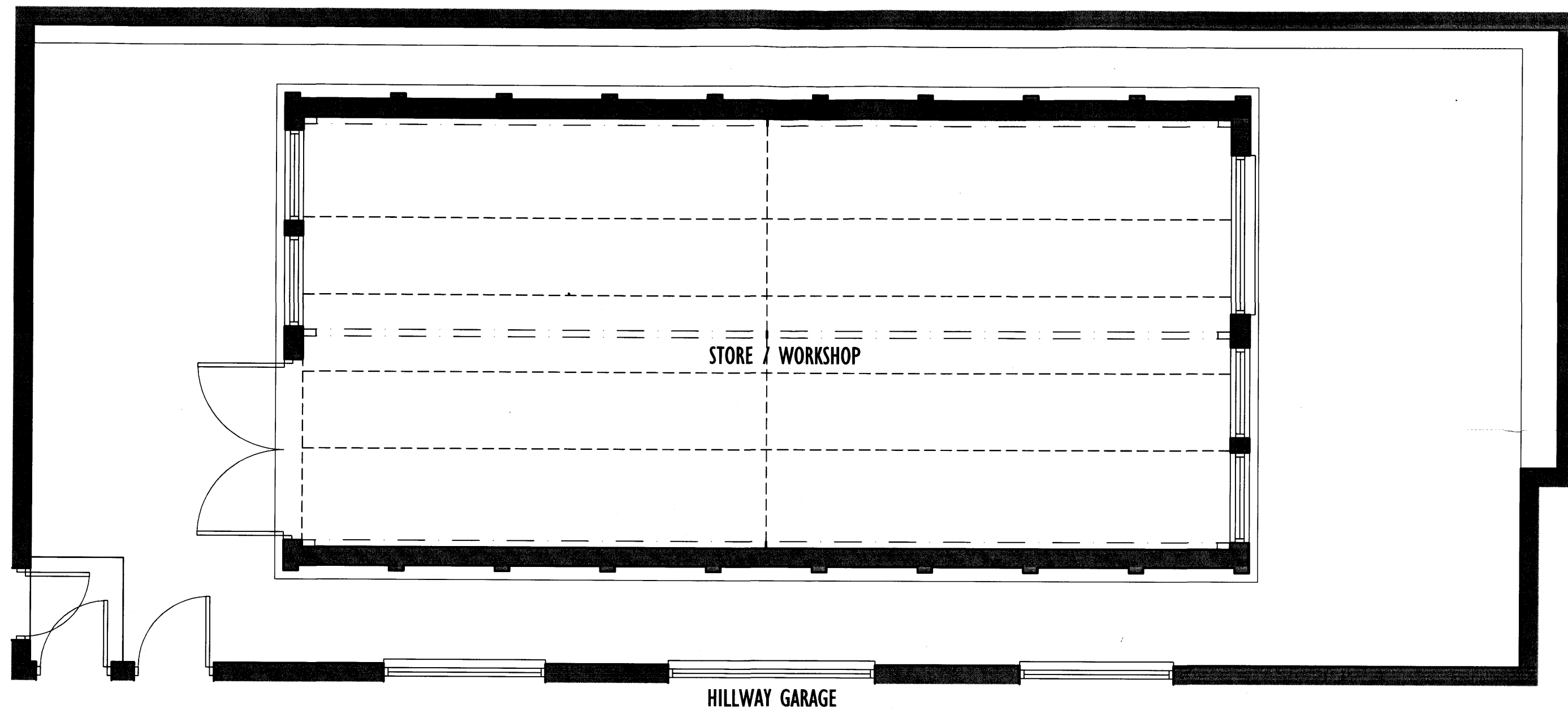
EXISTING FLOOR PLAN
