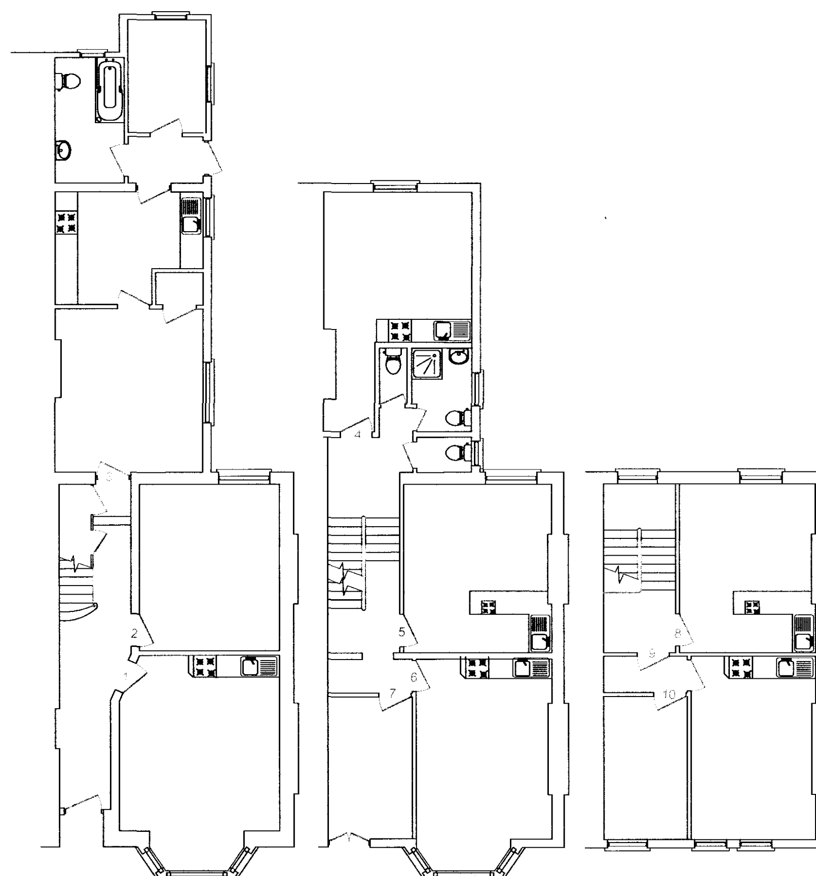
Ground Floor
